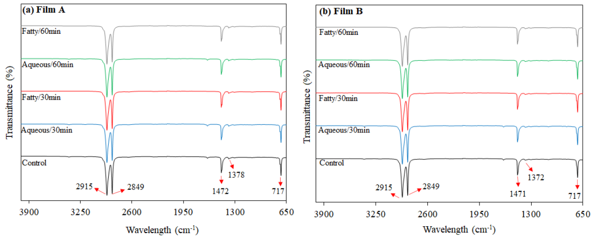
Figure 3. FT-IR spectra of inner layer of different packaging materials processed by ultrasound. (a) Film A: PE/PA/PE and (b) Film B: PE/PA/PE/PA/PE.
