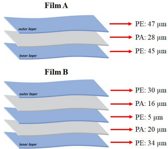
Figure 1. Composition of PE and PA multilayer films and their respective thicknesses.
