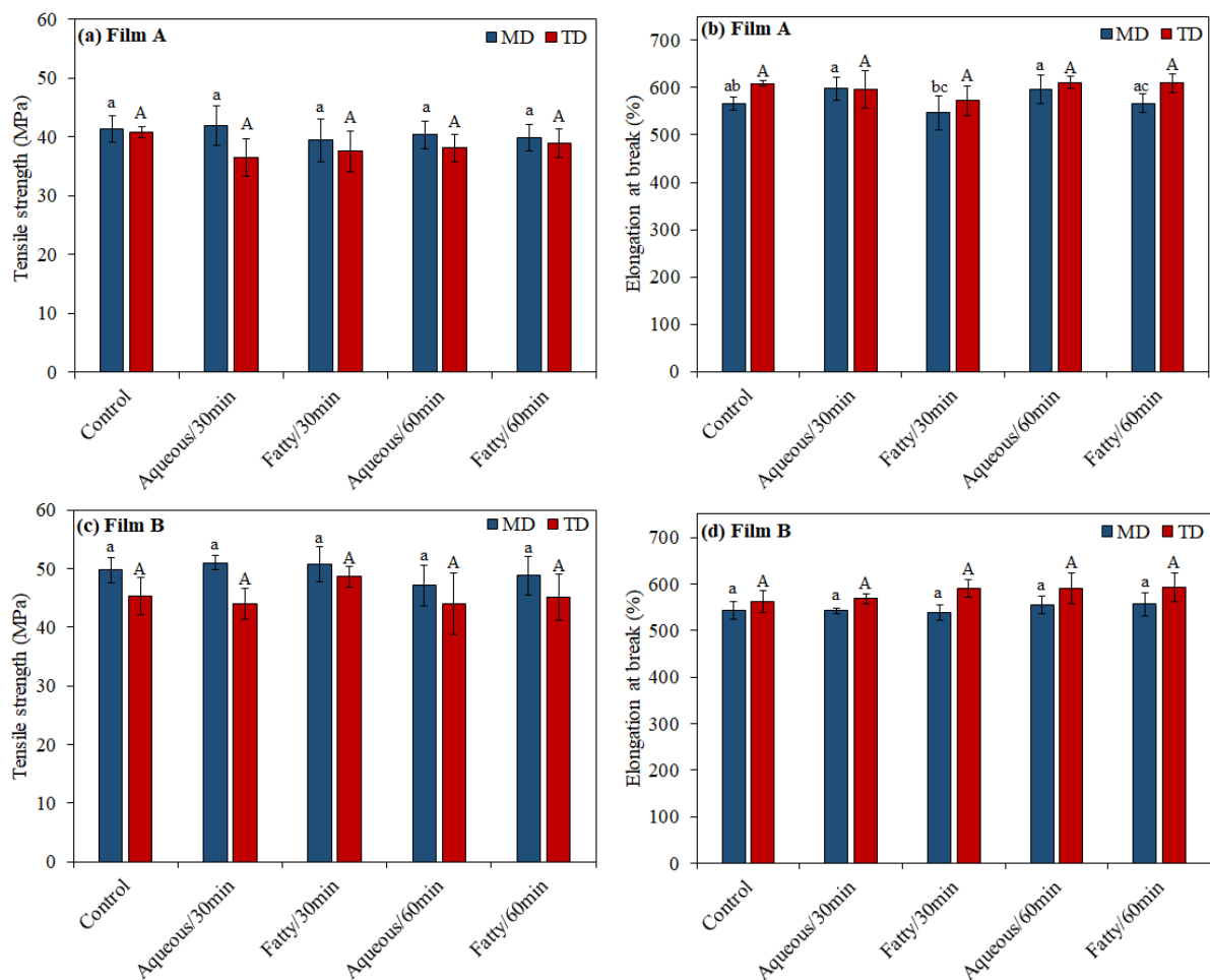
Figure 6. Tensile strength (MPa) (a) and (c) and elongation at break (%) (b) and (d) of different packaging materials processed by ultrasound. (a) and (b) Film A: PE/PA/PE, (c) and (d) Film B: PE/PA/PE/PA/PE, MD: machine direction and TD: transverse direction.
