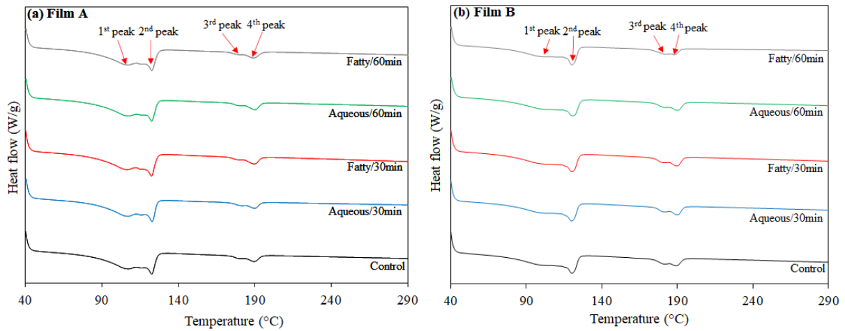
Figure 5. Differential Scanning Calorimetry of different packaging materials processed by ultrasound. (a) Film A: PE/PA/PE and (b) Film B: PE/PA/PE/PA/PE.
