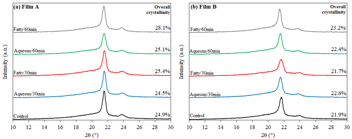
Figure 4. X-ray diffraction patterns of different packaging materials processed by ultrasound. (a) Film A: PE/PA/PE and (b) Film B: PE/PA/PE/PA/PE.
