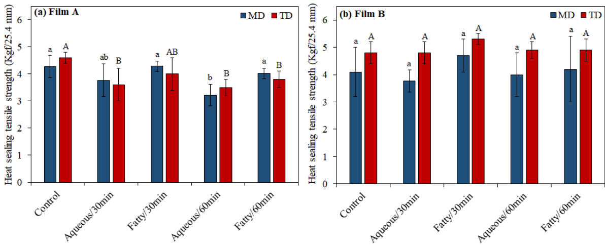
Figure 7. Heat sealing tensile strength of different packaging materials processed by ultrasound. (a) Film A: PE/PA/PE, (b) Film B: PE/PA/PE/PA/PE, MD: machine direction and TD: transverse direction.
