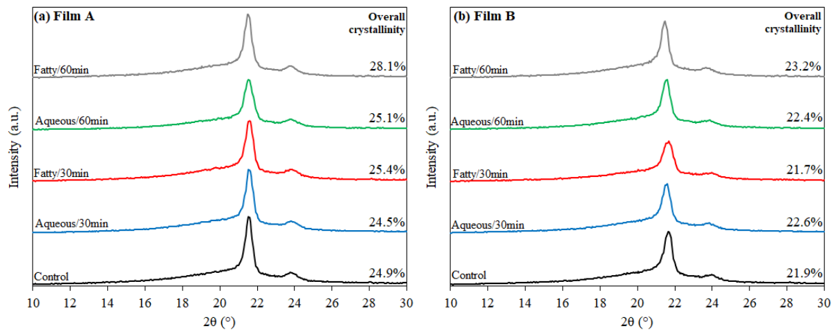
Figure 4. X-ray diffraction patterns of different packaging materials processed by ultrasound. (a) Film A: PE/PA/PE and (b) Film B: PE/PA/PE/PA/PE.
