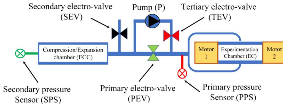
131 Figure 2 : Schematic view of the experimental set-up.
