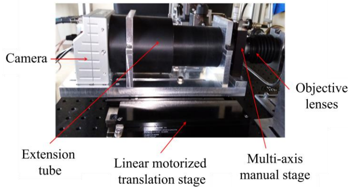
153 154 Figure 4 : View of the microscope and optical tomography system.
