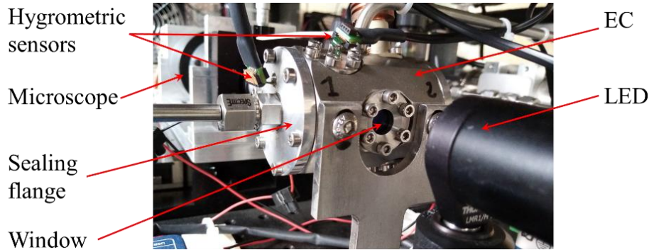
134 135 Figure 3 : Photograph of the EC assembly. LED (foreground), EC (foreground), microscope (background). In this picture the motors used 136 for Von Karman swirling flow generation are not mounted.
