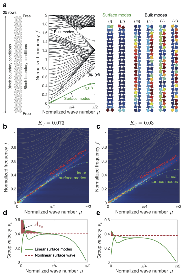
Figure 3. (a) 1D band structure showing bulk bands (black lines) and edge bands (green lines). Modal deformation fields of surfaces ( i-ii ) and bulk ( iii-vi ) modes. The colors indicate the rotation of each unit (with dark blue corresponding to no rotation and dark red to maximum rotation). (b)-(c) Comparison between the linear modes and the dispersion curves extracted from the nonlinear pulses reported in Figs. 2f and 2g via a double Fourier transform (from space-time to wave number-frequency) for (b) K_\theta = 0.073 and (c) K_\theta = 0.03 . (d)-(e) Group velocity of the nonlinear (red lines) and linear (green lines) surface waves for (d) K_\theta = 0.073 and (e) K_\theta = 0.03 .
