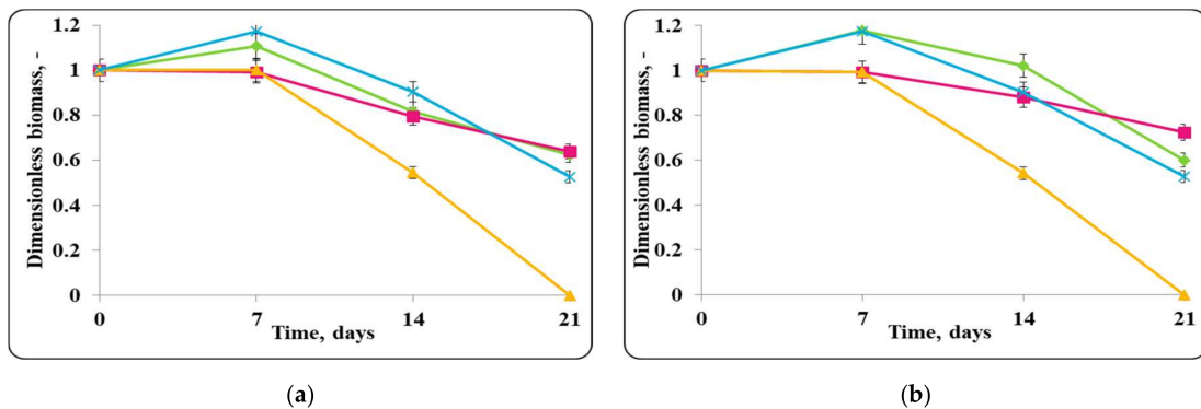
Figure 10. (a) free lactobacilli cells; (b) encapsulated lactobacilli cells. Changes in the dimensionless biomass of Lb. helveticus 2/20 and S. aureus ATCC 25923 in chocolate mouse at 4 \pm 2 °C. Legend: Green ◆ : Lb. helveticus 2/20 population following its inoculation; Pink ■ : Lb. helveticus 2/20 population following its co-inoculation with S. aureus ATCC 25923; Blue × : S. aureus ATCC 25923 population following its direct inoculation; Yellow ▲ : S. aureus ATCC 25923 population following its co-inoculation with Lb. helveticus 2/20.
