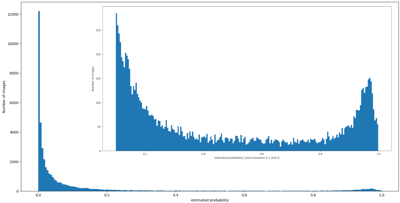
Figure 4. Probability repartition of the predictions made on our dataset using a YOLO-based classifier
