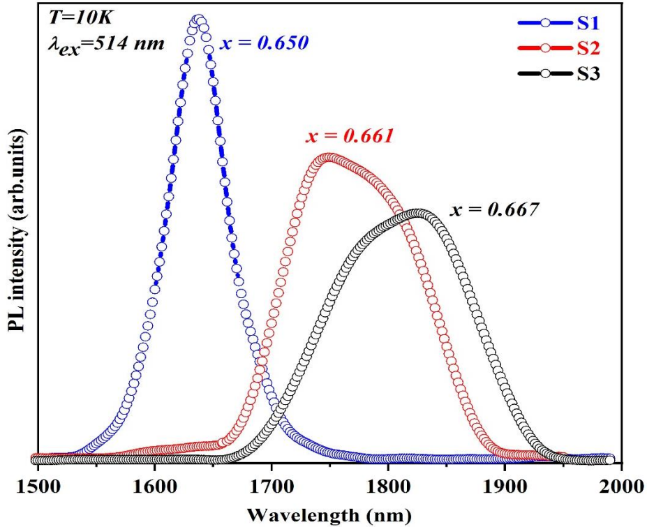
Figure 4: Comparison of the PL spectra of the three InGaAs samples with different In concentrations at 10K.
