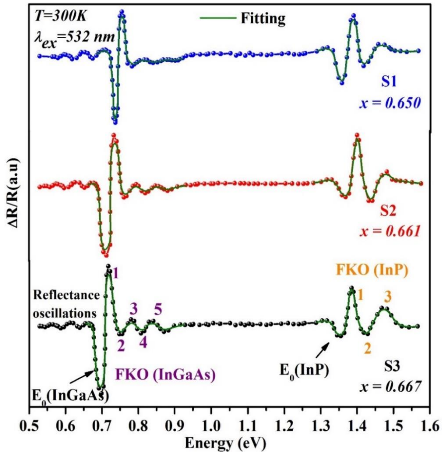
Figure 2: Room temperature PR spectra (dots) obtained from samples S1, S2 and S3 at different indium concentration and fits (green lines) performed using Eq. ~1.
