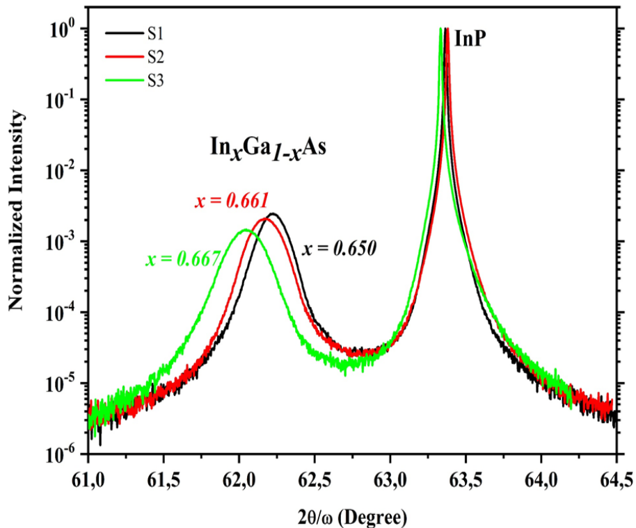
Figure 1: 2\theta/\omega HR-XRD spectra of the \text{In}_x\text{Ga}_{1-x}\text{As} layers having different In alloys grown on InP by MOVPE [7].
