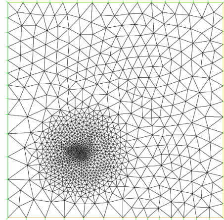
FIGURE 2. Mesh at t = 0.241
