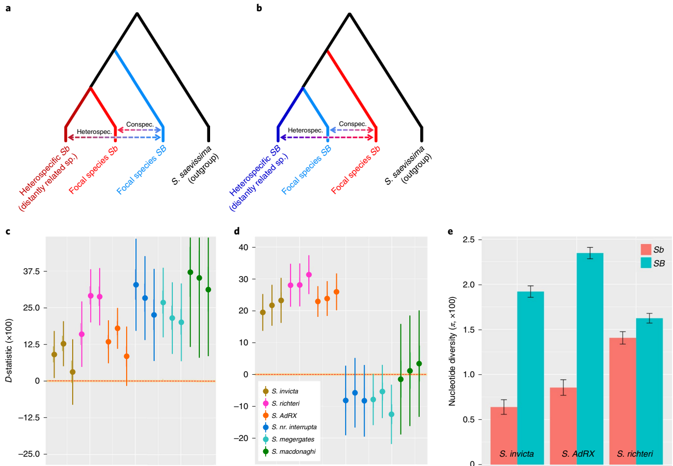
Fig. 5 | Results of ABBA/BABA tests ( D -statistics) for recombination (gene flux) between conspecific Sb and SB haplotypes and estimates of nucleotide diversity ( \pi ). a, b , ABBA/BABA tests were performed for each of the six socially polymorphic Solenopsis study species to detect gene flux from SB into conspecific Sb haplotypes by comparing focal SB males to conspecific and heterospecific Sb males ( a ) and to detect gene flux in the opposite direction by comparing focal Sb males to conspecific and heterospecific SB males ( b ). c , Gene flux from SB into conspecific Sb haplotypes; for each of the six species, D -statistics from the ABBA/BABA tests were computed by using Sb haplotypes from each of the three most distantly related species for the heterospecific comparisons (that is, for each species there are three points of the same colour indicating the values of these three estimates). Error bars indicate \pm 3 s.e.m. estimated with a weighted-block jackknife approach using 50-kb blocks of the complete supergene region; non-overlap with zero signifies a statistically significant D -value (evidence for gene flux). d , Gene flux from Sb into conspecific SB haplotypes was measured as in c but with SB males used as referents to estimate gene flow in the opposite direction. e , Nucleotide diversity ( \pi ) within the supergene region for Sb and SB males of the three best-sampled species (native ranges); error bars indicate the 95% CIs about the means derived from resampling of 228 non-overlapping 50-kb windows. Nucleotide diversity was significantly lower in Sb than SB males in each of the species ( t -tests, all P < 0.001 ). The relatively modest difference in diversity between Sb and SB in S. invicta (as well as the other two species), stands in stark contrast to the extreme reduction in Sb diversity relative to SB diversity in invasive S. invicta portrayed in Pracana et al. 28
