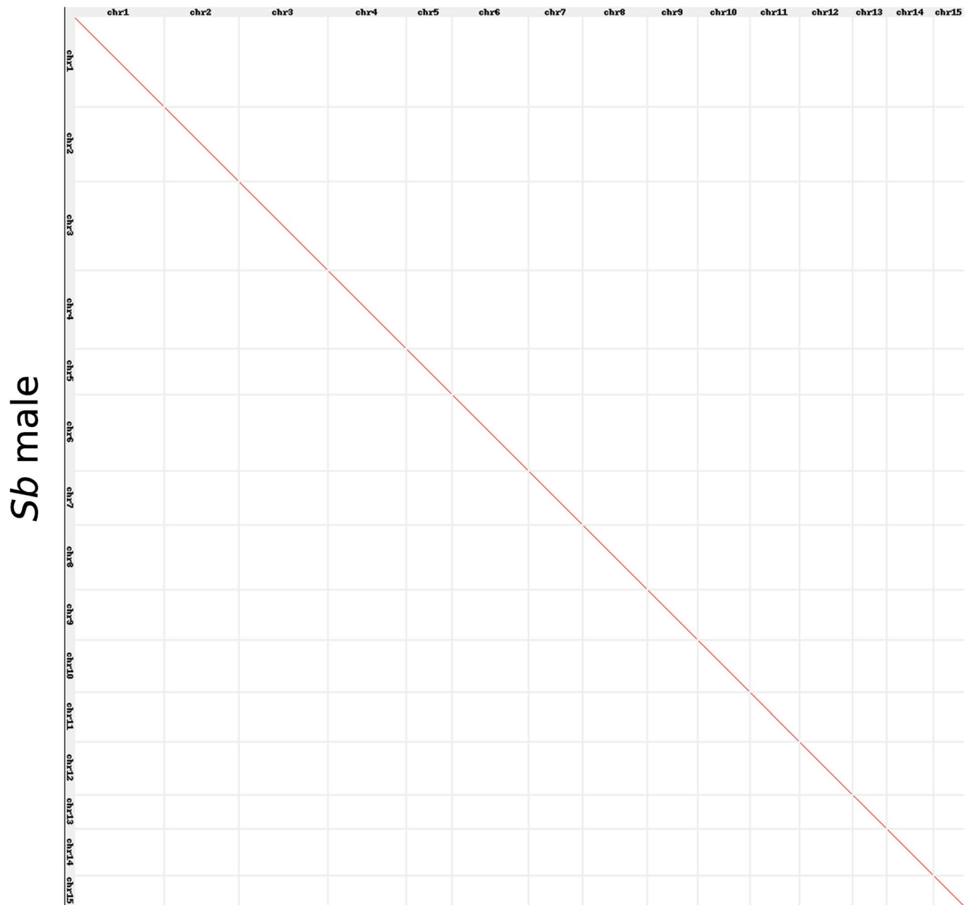
Extended Data Fig. 1 | Dot plot of the alignment between chromosomes 1-15 of Sb and SB males of S. invicta from the invasive (United States) range. The red line indicates the forward strand alignment.
