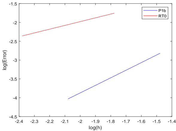
FIGURE 1. Pressure error with respect to the mesh size.
