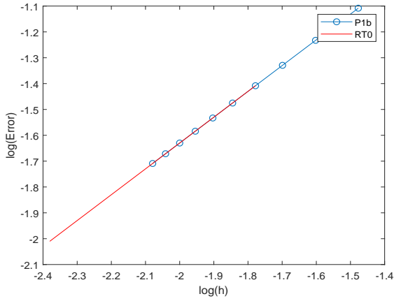
FIGURE 3. Concentration error with respect to the mesh size.
