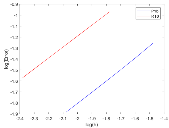
FIGURE 2. Velocity error with respect to the mesh size.
