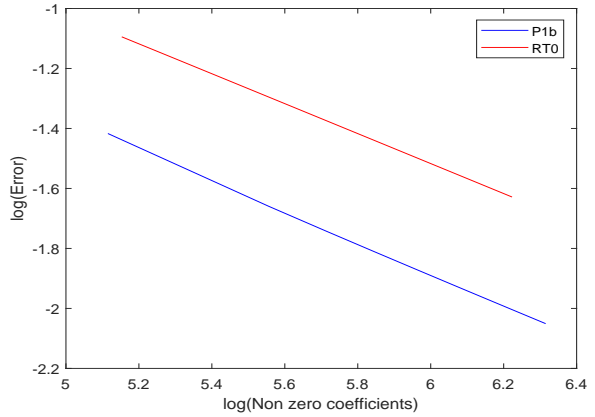
FIGURE 6. Total relative error with respect to the number of non-zero coefficients in the matrices.
