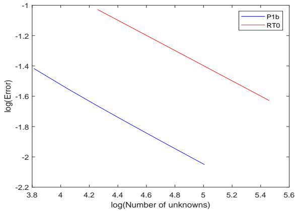
FIGURE 5. Total relative error with respect to the number of unknowns.
