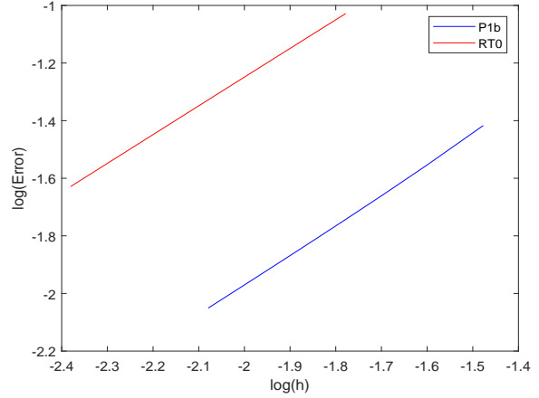
FIGURE 4. Total relative error with respect to the mesh size.
