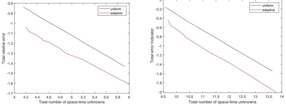
FIGURE 5. left: Total relative errors err . Right: Total error indicators E_{total} .
