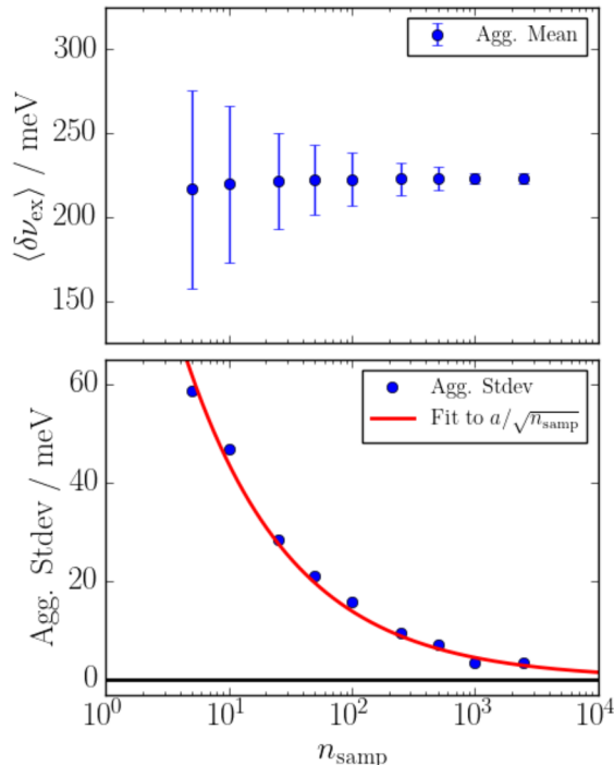
Figure 12: Top: Aggregate means of the ensemble average transition energy shift \langle \delta\nu_{\text{ex}} \rangle vs. n_{\text{samp}} . Error bars are the aggregate standard deviation. Bottom: Aggregate standard deviations vs. n_{\text{samp}} . The red curve is a fit to a/\sqrt{n_{\text{samp}}} where a = 139 meV.
