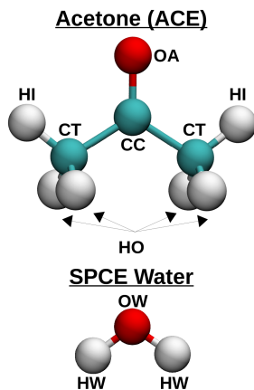
Scheme 1: Space-filling models and atom labels of all simulated systems.
