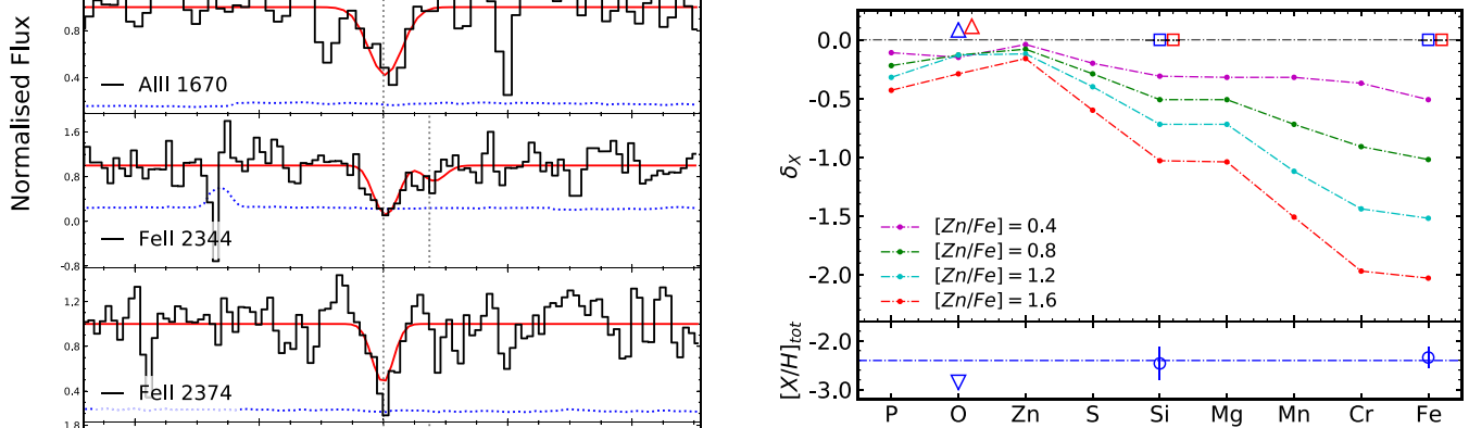
Figure 5. Dust depletion pattern and metallicity for the measured column densities of the features found in absorption in the afterglow of GRB 160410A. Top panel: Dust depletion sequence for GRB 160410A. Squares (top panel) and circles (bottom panel) denote the Si and Fe lines meanwhile triangles refer to the limits we derive for the saturated O line. With a small offset for visualization purposes. The red squares denote the depletion \delta_X values obtained for the common velocity component to all the elements observed, blue squares are the depletion considering the total column density measured. For comparison, we plot with a dash-dotted line in different colours the dust depletion sequence obtained from the fitting of QSO-DLA absorption systems in De Cia et al. (2016). Bottom panel: Corresponding metallicity for the observed ions considering all the velocity components. The mean metallicity is shown with a dashed-dotted line.
