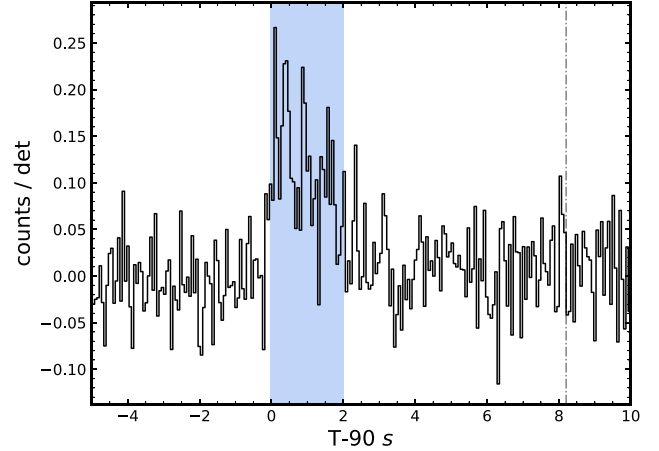
Figure A1. BAT mask-weighted light curve in the 15 to 350 keV range of GRB 160410A with 64 ms binning. The blue area marks a multi-peaked structure during the first two seconds. The dash-dotted line marks the end of the T_{90} duration from Sakamoto et al. (2016) in the same energy band.
