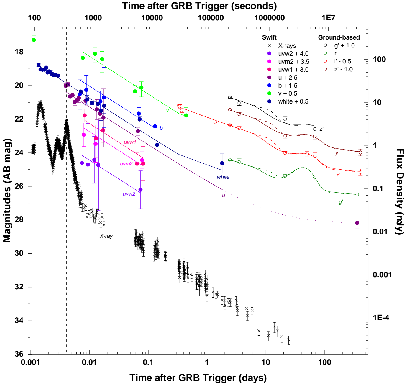
Fig. 1. Observations of optical transient that followed GRB 140506A. UVOT data ( uvw2 , uvw1 , u , b , v , white ) are presented in this paper (Table A.1). Ground-based u'g'r'i'z' magnitudes are from Fynbo et al. (2014) and Heintz et al. (2017). The downward-pointing triangle in g' at 68 days is an upper limit. We do not show UVOT upper limits and JHK s data as they add no relevant information. Data are corrected for Galactic extinction, given in the AB magnitude system, and additionally offset by the values given in the legend to improve legibility. The flux density scale is only valid for the (unshifted) r' band. The rest was shifted for clarity. The scale of the X-ray data was chosen arbitrarily. We show two possible fits with breaks at 7 (solid fit curve) and at 12 (dotted fit curve) days, which include both the afterglow and the SN/host contributions. Dotted vertical lines mark the peaks of two early X-ray flares that have no counterparts in the UV/optical range, whereas the flare marked by the dashed vertical line is also detected by UVOT. The flatter decay after 0.33 d in the late UVOT v and white light curves is simply the shifted r' -band fit (see text for more details).
