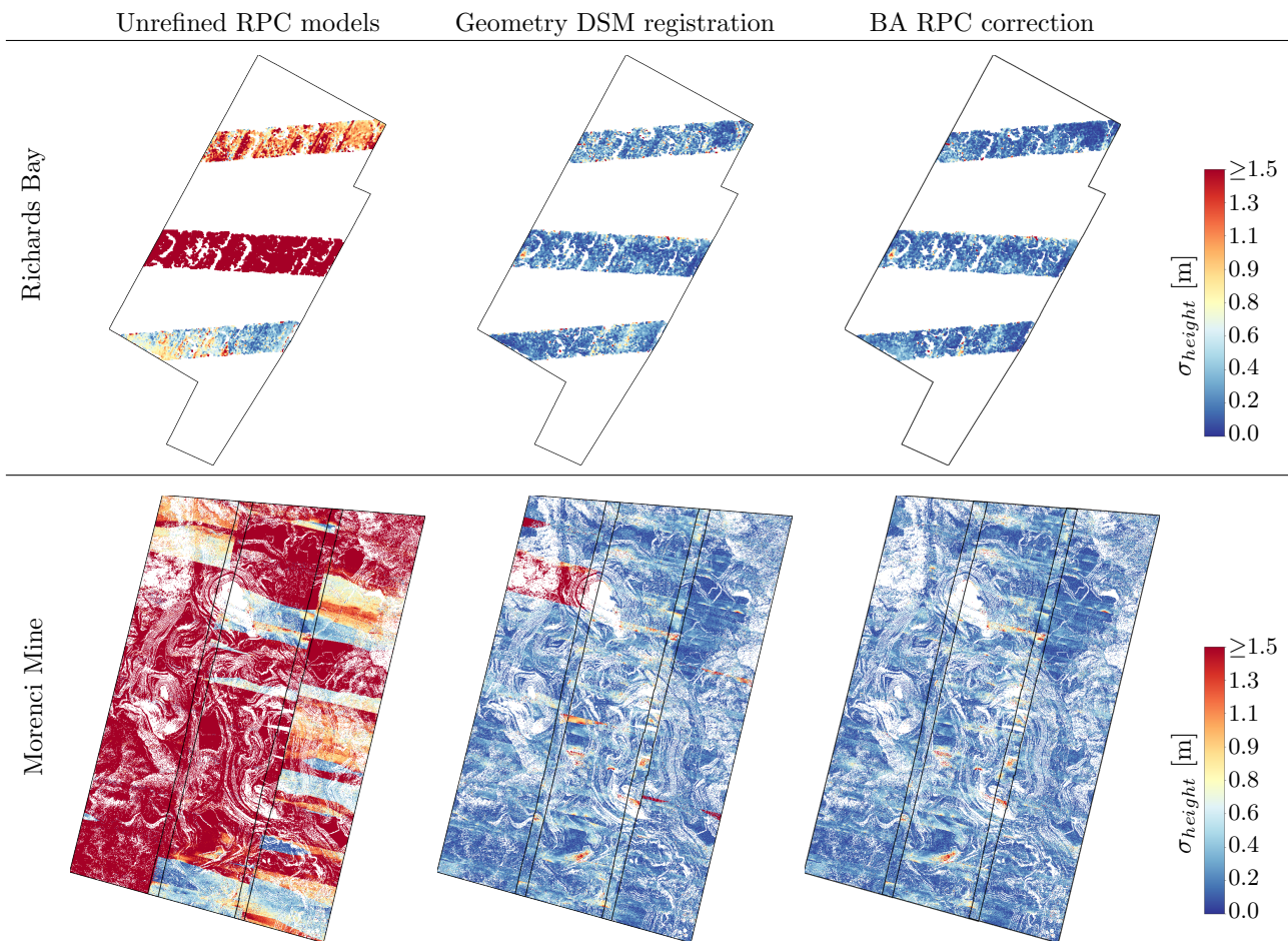
Figure 11: Deviation of corresponding DSM height values, \sigma_{\text{height}} , for an acquisition date of each time series. 144 DSMs from different stereo pairs are used to cover the Morenci Mine AOI (48 DSMs for each sensor strip), while 4 pairwise DSMs are enough for the smaller AOI in Richards Bay. \sigma_{\text{height}} is computed where at least two pairwise DSMs overlap, which only occurs in some bands for Richards Bay. Geometry registration after depth from stereo fails to align some DSMs near the top-left corner of the Morenci Mine, which is corrected when bundle adjusted RPCs are used to compute the models.
