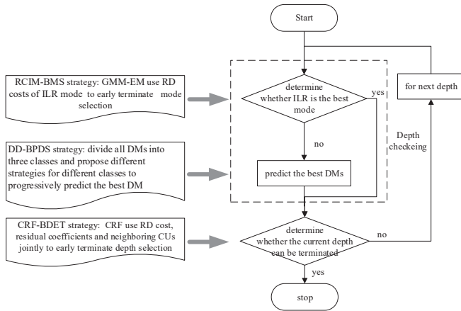
Fig. 1: Overview of the Proposed Algorithm.
