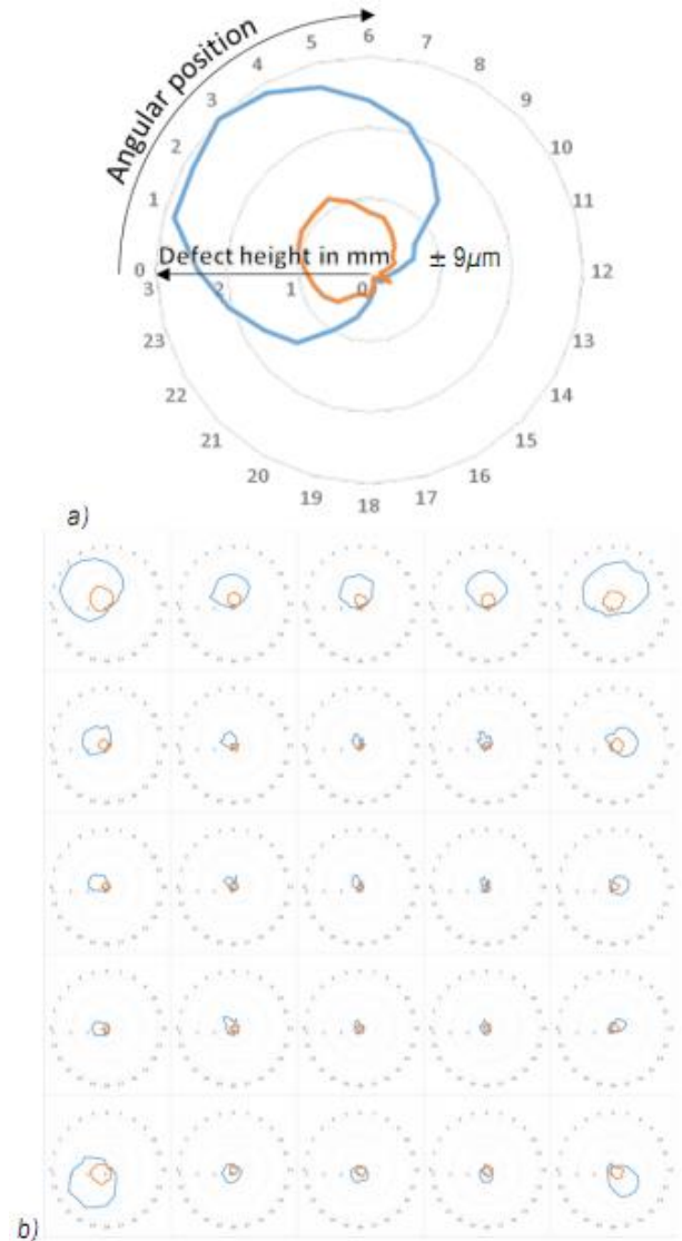
Fig. 9 a) Example and b) defect cartography of the massive specimen (blue: \varnothing 30 mm, orange: \varnothing 20 mm)
