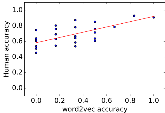
(d) Correlation between human responses and the accuracy of the offset method (each point represents a source + domain pair)
