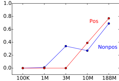
Figure 3: Effect of training corpus size (in sentences) on the accuracy of the analogy task, averaged across vector and window size settings.
