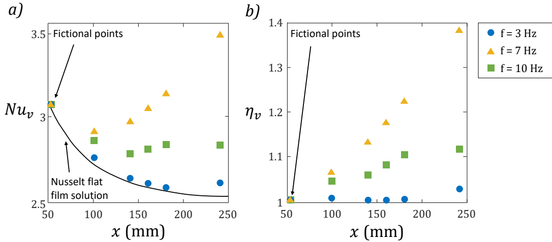
Figure 12: Spatial evolution of the Nusselt number \overline{Nu}_v (a) and \eta_v (b) along the liquid film for three perturbation frequencies f for Re = 200 , \beta = 10^\circ and q_w = 1.25 W/cm 2 . The black line represents the Nusselt flat film solution.
