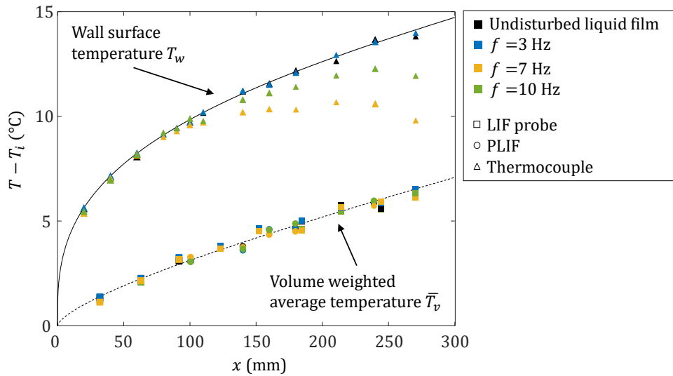
Figure 10: Spatial evolution of the volume weighted average temperature of the liquid film \overline{T}_v and T_w the wall surface temperature. Comparison to the theoretical model for the undisturbed flat liquid film in dotted and solid lines respectively, with Re = 200 , \beta = 10^\circ and q_w = 1.25 \text{ W/cm}^2 .
