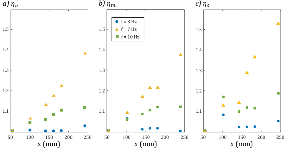
Figure 13: Spatial evolution of the efficiency factor \eta calculated with the three previously defined film temperature T_m , T_v and T_s . Same experimental conditions as in Fig. 12. As in Fig. 12, the points at x = 50 mm were hand placed to help read the trends.
