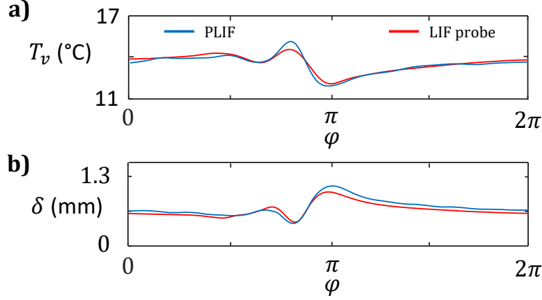
Figure 6: Comparison of the average temperature T_v (a) and the film height \delta (b) measured with the PLIF technique and the LIF probe ( Re = 200 , \beta = 10^\circ , x = 160 mm, f = 10 Hz, T_i = 10 °C and q_w = 1.25 W/cm 2 ).
