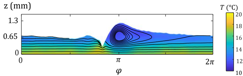
Figure A.1: Stream lines of the flow in the liquid film under a wave obtained using the Kapitza-Shkadov model used for the velocity calculation, printed over the temperature field measured by PLIF. Results for Re = 200 , \beta = 10^\circ , f = 10 Hz, x = 160 mm, T_i = 10^\circ\text{C} and q_w = 1.25 W/cm 2
