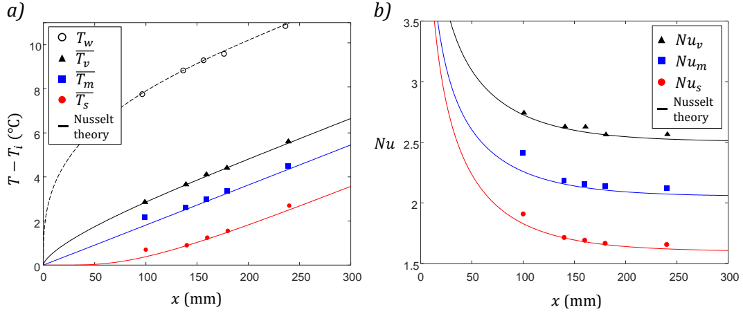
Figure 11: Spatial evolution of the time-averaged values of the temperatures \overline{T}_m , \overline{T}_v and \overline{T}_s (a) and their corresponding values of the Nusselt number: \overline{Nu}_m , \overline{Nu}_v and \overline{Nu}_s (b). Measurements, in dots, are provided by PLIF images of the temperature field inside a film generated in the conditions: f = 3 Hz, for Re = 200 , \beta = 10^\circ and q_w = 1.25 W/cm 2 . The lines are extracted from the Nusselt theory in the same configuration as the experiments.
