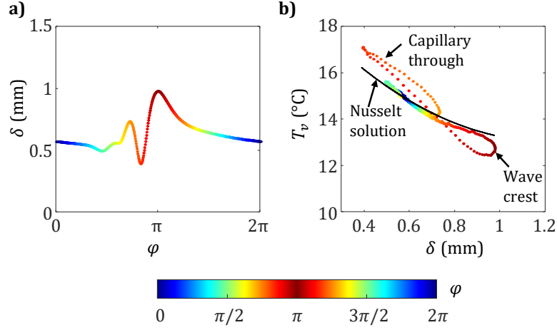
Figure 19: Evolution of the thickness \delta (a) and the volume average temperature T_v (b) during the period of a wave. The conditions correspond to f = 10 Hz, Re = 200 , \beta = 10^\circ , T_i = 10^\circ\text{C} and q_w = 1.25\text{ W/cm}^2 and x = 180 mm. The black curve is for the theoretical model based on the Nusselt solution which allows to determine the average temperature in the film cross-section in the absence of mixing by the wave.
