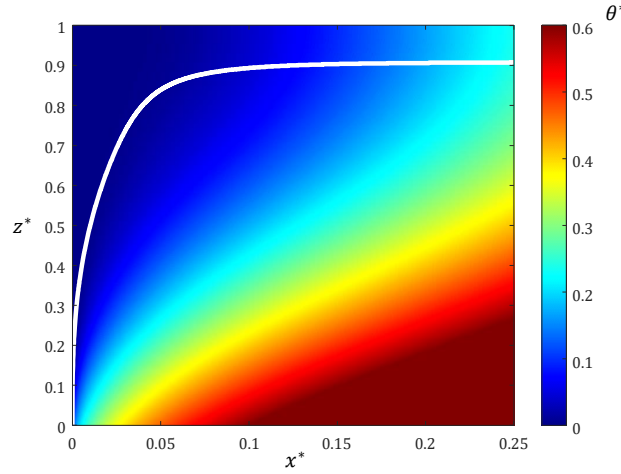
Figure 3: Growth of the thermal boundary layer (white line) superimposed to the solution of the theoretical Nusselt flat film solution represented in dimensionless variables under adiabatic condition at the free surface.
