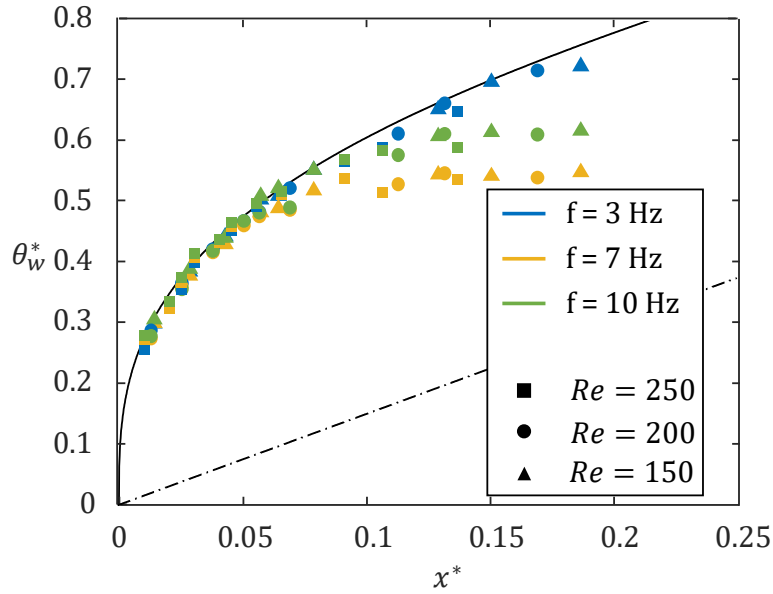
Figure 15: Spatial evolution of the non-dimensional wall temperature \theta_w^* for three values of the Reynolds number Re and three perturbation frequencies f as represented on graphs (a), (b) and (c) of Figure 14. The dotted line represents the liquid film temperature \theta_m^* .
