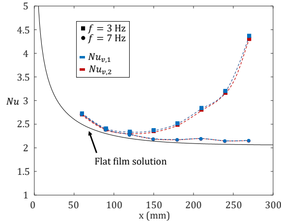
Figure A.2: Comparison of the two time-averaging methods used to evaluate the Nusselt number. The first method based on Equation (20) is plotted in blue, while the second method based on Equation (21) is plotted in red. The results correspond to two wave frequencies ( f = 3 Hz and f = 7 Hz) and were obtained for Re = 200 , \beta = 10^\circ and q_w = 1.25 W/cm 2 .
