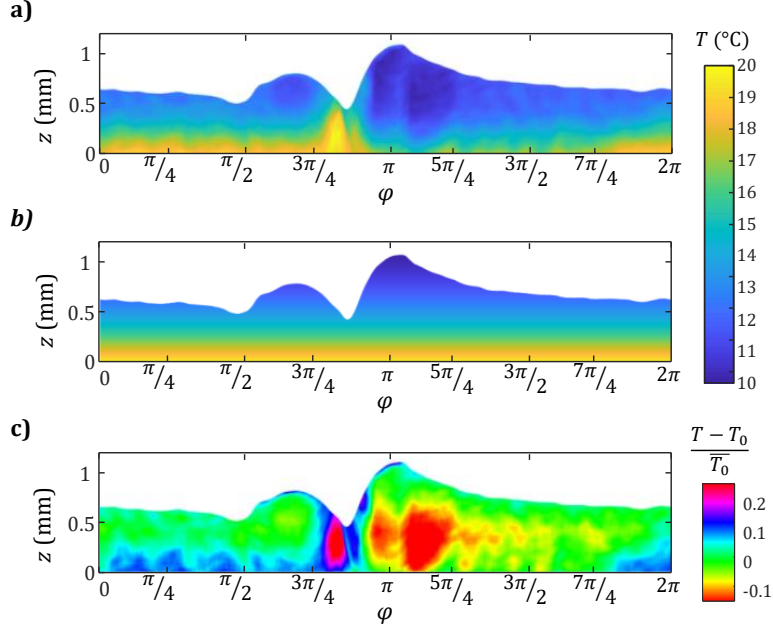
Figure 17: Temperature field T in the film obtained using PLIF measurement technique (a) and the corresponding temperature field T_{Nu} calculated with the extrapolated Nusselt solution under the assumption of pure diffusion in the transverse direction (b). The normalized difference between T and T_{Nu} is shown in (c). Results correspond to Re = 200 , \beta = 10^\circ , x = 180 mm, f = 10 Hz and T_i = 10 °C.
