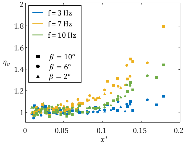
Figure 16: Evolution of the efficiency factor \eta_v obtained experimentally with the dimensionless distance x^* . The data covers the totality of the studied Re , \beta and f values.
