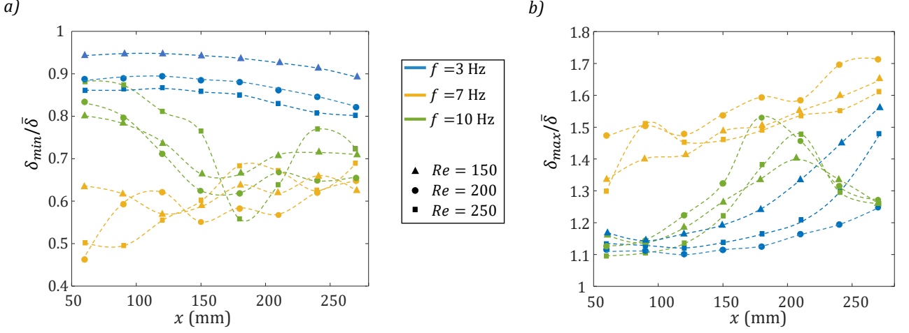
Figure 8: Evolutions of the minimum (a) and maximum (b) of the film thickness as a function of the distance x from the flow inlet. Measurements obtained with the LIF probe for three values of the Reynolds number: Re = 150 ( \triangle ), Re = 200 ( \circ ) and Re = 250 ( \square ), and \beta = 10^\circ , T_i = 10^\circ\text{C} and q_w = 1.25\text{ W/cm}^2 . The dotted curves were hand drawn to help reading.
