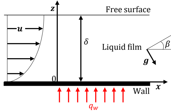
Figure 2: Parameters used for the flat liquid film model.
