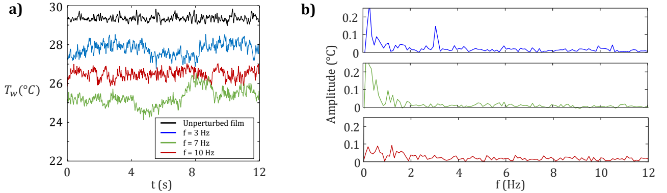
Figure 7: Variations in wall temperature during the passage of waves at different frequencies measured with Re = 200 , \beta = 10^\circ , x = 250 mm, T_i = 15 °C and q_w = 1.25 W/cm 2 . Raw data are presented in (a) and their corresponding FFT are presented in (b). The difference in wall temperature between the different cases is a consequence of heat transfer.
