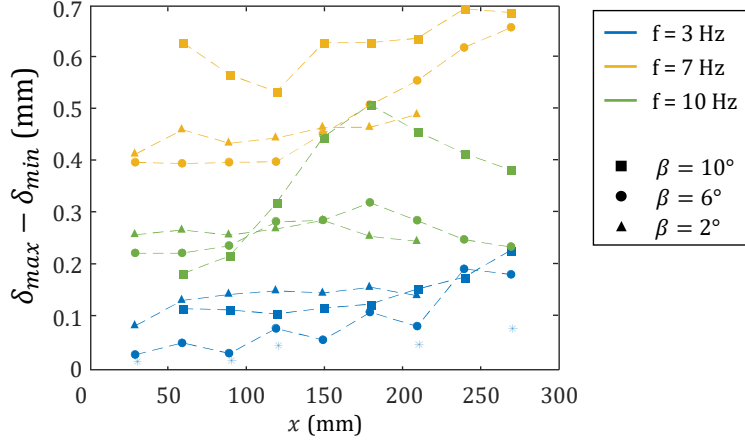
Figure 9: Spatial evolution of the amplitude of the waves for three perturbation frequency f = 3\text{ Hz} , f = 7\text{ Hz} and f = 10\text{ Hz} represented along the flow distance x . The measurements are represented for Re = 200 and q_w = 1.25\text{ W/cm}^2 . The dotted curves were hand drawn to help reading.
