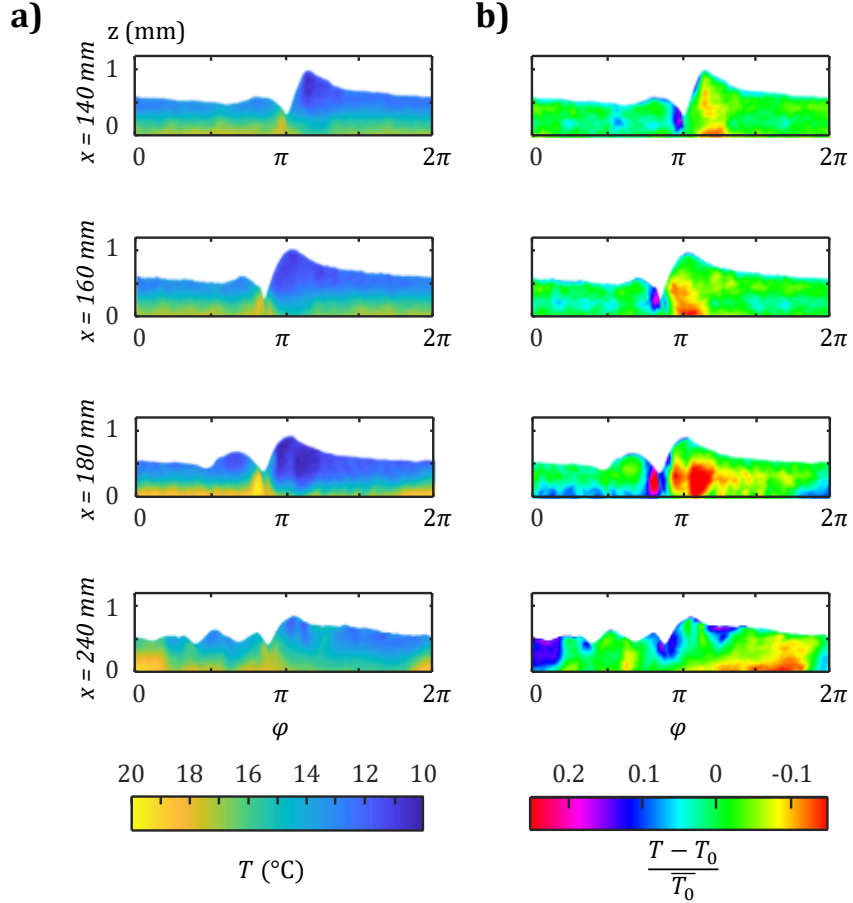
Figure 18: Spatial evolution of the temperature field T (a) and of the normalized difference between T and T_{Nu} (b) along the flow of the film. Results were obtained for Re = 200 , \beta = 10^\circ , f = 10 Hz and T_i = 10^\circ\text{C} .
