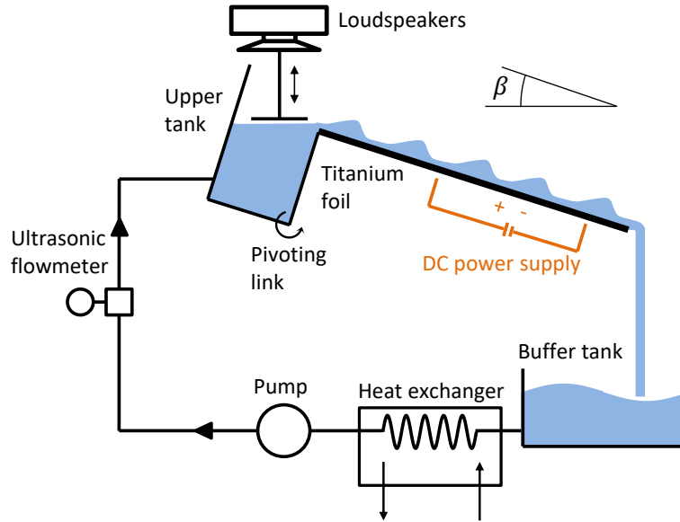
Figure 4: Set-up used for the generation of the waves and the heating of the falling liquid film.
