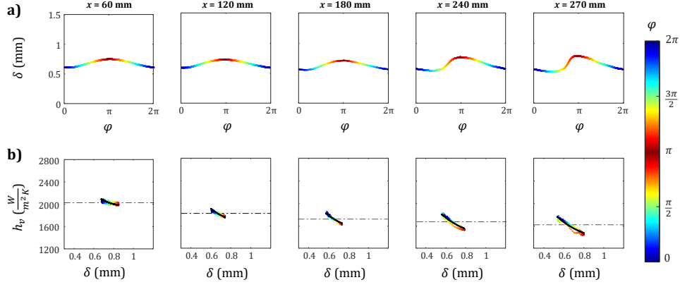
Figure 20: Evolution of the thickness \delta (a) and the heat transfer coefficient h_v (b) of the falling liquid film compared to the pure diffusion model (black line). The color of the curves is matched in phase between the two rows. The horizontal dotted line is the time average heat transfer coefficient calculated from the experimental data from the LIF probe. Results for f = 3 Hz, \text{Re} = 200 , \beta = 10^\circ , T_i = 10^\circ\text{C} and q_w = 1.25 \text{W}/\text{cm}^2 .
