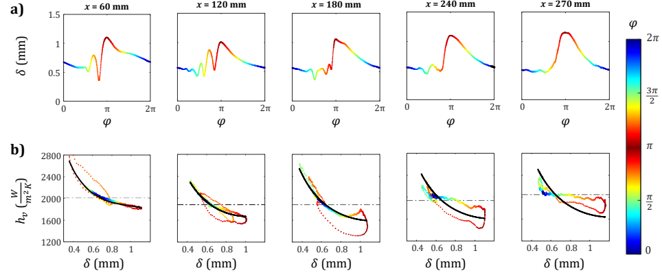
Figure 21: Evolution of the thickness \delta (a) and the heat transfer coefficient h_v (b) of the falling liquid film compared to the pure diffusion model (black line). The color of the curves is matched in phase between the two rows. The horizontal dotted line is the time average heat transfer coefficient calculated from the experimental data from the LIF probe. Results for f = 7 Hz, \text{Re} = 200 , \beta = 10^\circ , T_i = 10^\circ\text{C} and q_w = 1.25 \text{W}/\text{cm}^2 .
