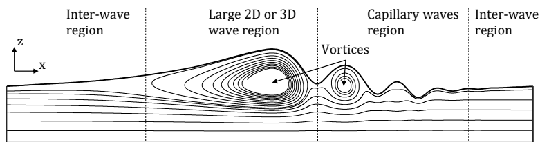
Figure 1: Topology of a wavy film with capillary waves flowing down an inclined plane.
