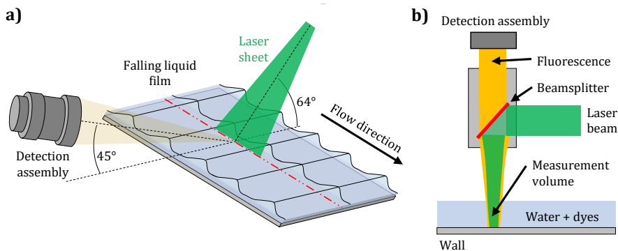
Figure 5: Optical configuration used for the LIF techniques applied to the falling film. a) Illumination by a laser sheet and detection by a camera assembly for the PLIF technique. b) Illumination and detection by the punctual LIF probe.
