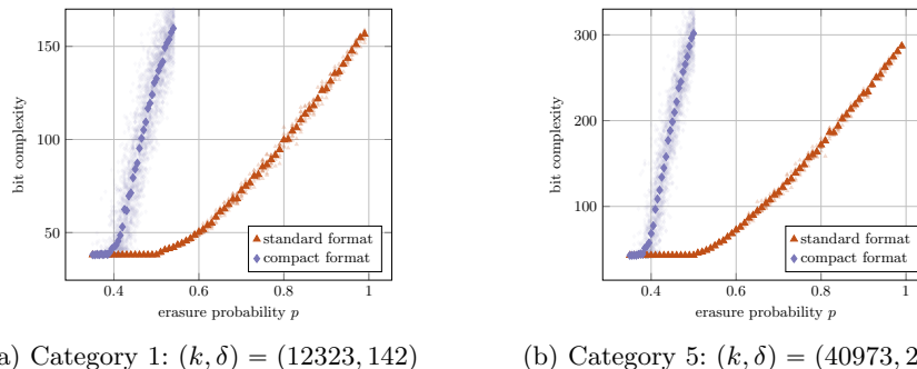
Fig. 1: Bit complexity of partial key exposure attack in the erasure model on the compact and standard key representations based on experiments.
