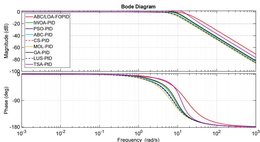
Figure 12. Bode plots comparison with existing techniques.
