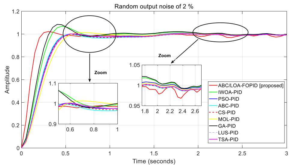
Figure 16. Controller's comparison with random output noise for 2% of the amplitude of the reference signal.
