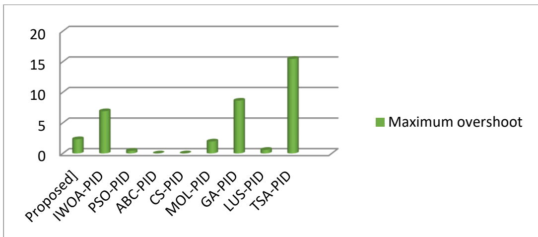
Figure 9. Percentage of overshoots for different techniques.
