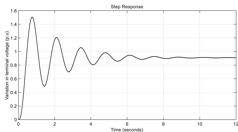
Figure 2. AVR system step response in the absence of a PID controller.
