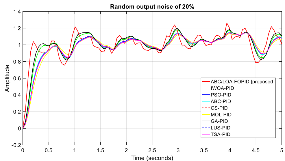
Figure 17. Controller's comparison with random output noise for 20% of the amplitude of the reference signal.
