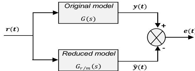
Figure 6. Error signal for model reduction.
