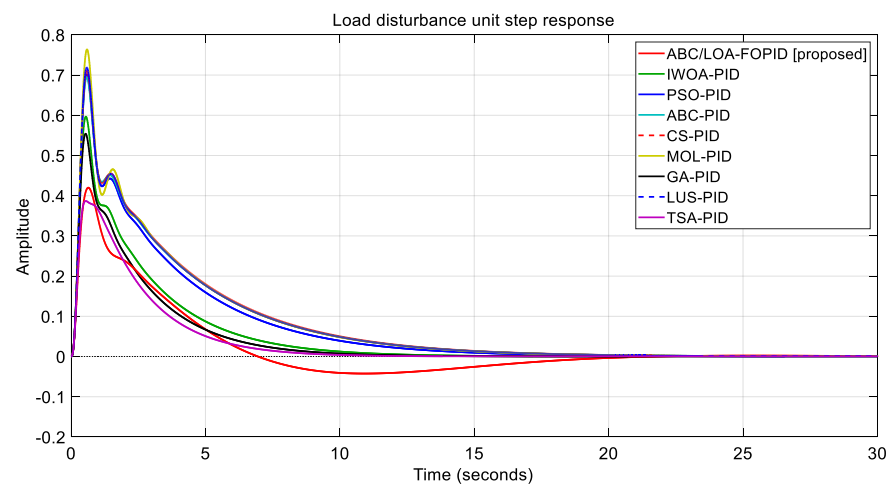
Figure 18. Disturbance rejection comparison for different techniques.
