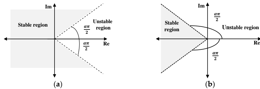
Figure 3. Stable regions when 0 < \alpha < 1 (a) and 1 < \alpha < 2 (b).
