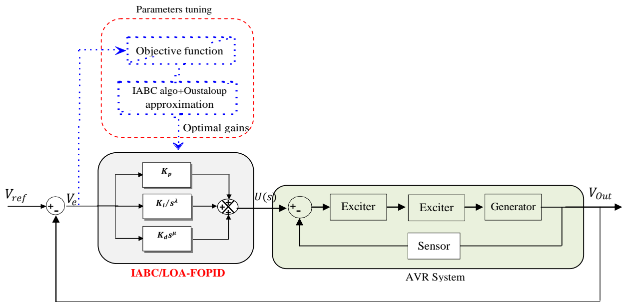
Figure 5. Proposed IABC/LOA-FOPID controller applied to the AVR system.
