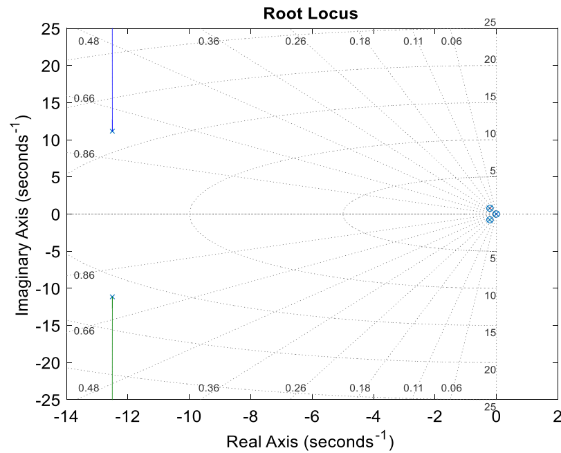
Figure 14. Root locus plot.
