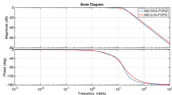
Figure 7. Bode diagram approximations.
