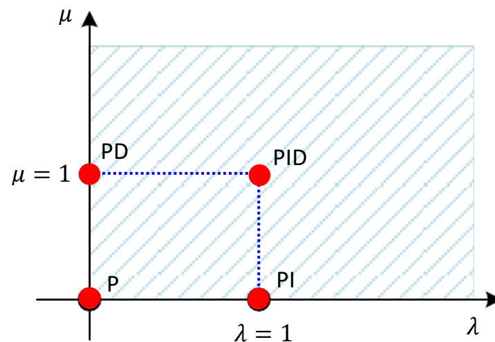
Figure 4. PID/PI λ D μ controllers' graphical representation.
