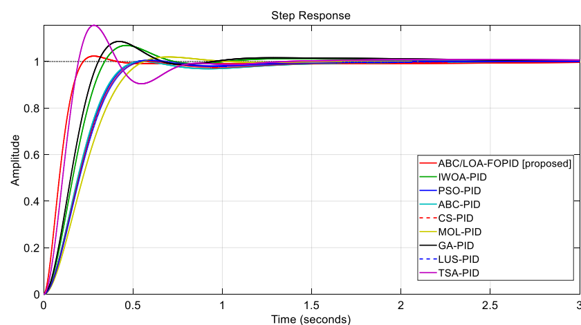
Figure 8. AVR terminal voltage comparison with existing techniques: IWOA-PID [21], PSO-PID [12], ABC-PID [15], CS-PID [26], MOL-PID [28], GA-PID [12], LUS-PID [31], and TSA [23].
