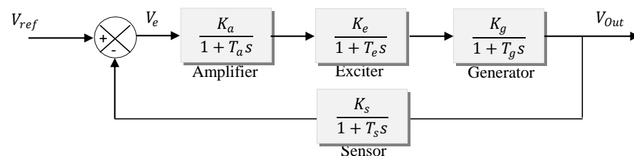
Figure 1. AVR system block diagram without a PID controller.
