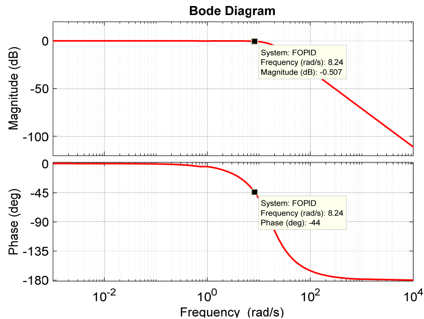
Figure 15. Bode plot.
