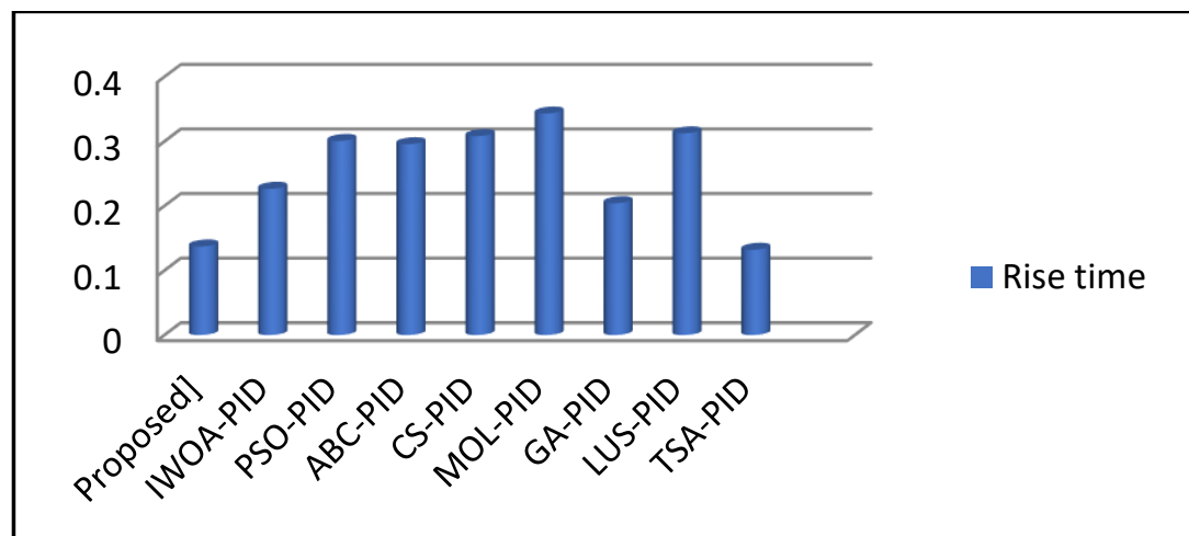
Figure 11. Rise times for different techniques.
