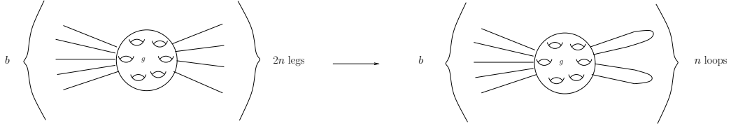
FIGURE 5.1. Trading 2n primitive insertions for n nodes
