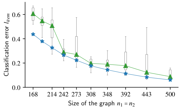
Fig. 6 Classification error with respect to the size of the data matrix (lower is better); ★ is the median of the conditional Bayes risk; ▲ is the median prediction error obtained by our algorithm.
