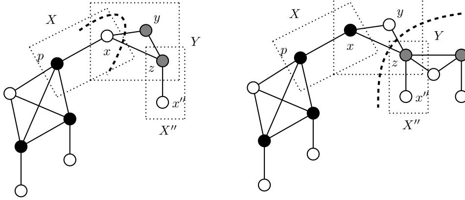
(b) The vertices to the left of the dashed curve represent those deleted from G to obtain G^* . G^* has twins x^* and y^* ; and G^* is a twin-free block graph. The black vertices constitute the set A \cup \{x^*\} and the grey vertices constitute an LTD-set S^* of G^* .
