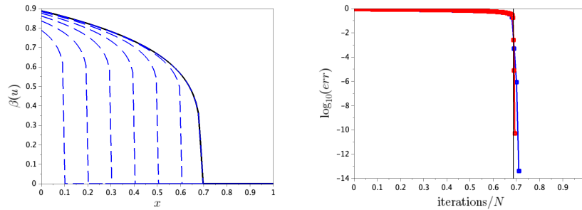
Fig. 1: Left: the solution for N = 100 (black) and the iterates \beta(u_n) of the Jacobi-Newton method for n = 10, 20, \dots, 70 . Right: convergence history of the Jacobi-Newton method for N = 100 (blue) and 400 (red), the iteration count is scaled by the size of the discrete system; the error is measured in l_\infty norm. The vertical black line positioned at N_f/N indicate the location of the solution front.
