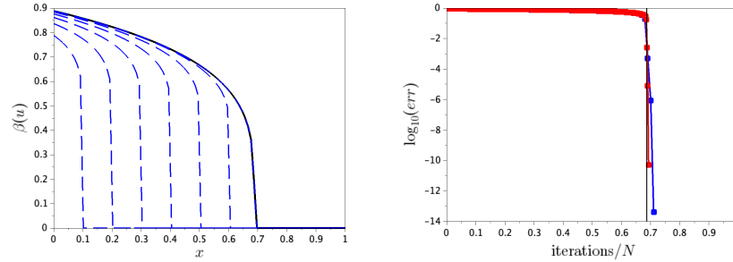
Fig. 1: Left: the solution for N = 100 (black) and the iterates u_n of the Jacobi-Newton method for n = 10, 20, \dots, 70 . Right: convergence history of the Jacobi-Newton method for N = 100 (blue) and 400 (red), the iteration count is scaled by the size of the discrete system; the error is measured in l_\infty norm. The vertical black line indicate the location of the solution front.
