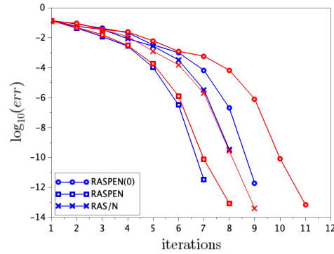
Fig. 2: Convergence history of preconditioned Newton's method for N = 100 (blue) and 400 (red); the error is measured in l_\infty norm.
