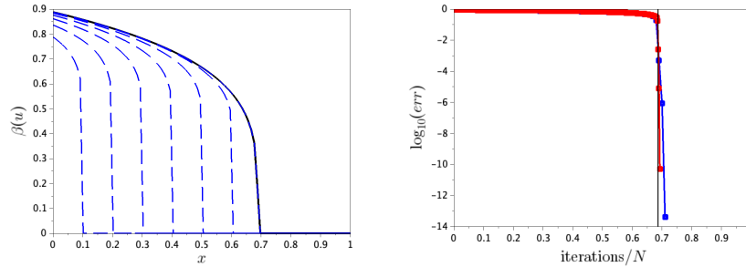
Fig. 1: Left: the solution for N = 100 (black) and the iterates \beta(u_n) of the Jacobi-Newton method for n = 10, 20, \dots, 70 . Right: convergence history of the Jacobi-Newton method for N = 100 (blue) and 400 (red), the iteration count is scaled by the size of the discrete system; the error is measured in l_\infty norm. The vertical black line positioned at N_f/N indicate the location of the solution front.
