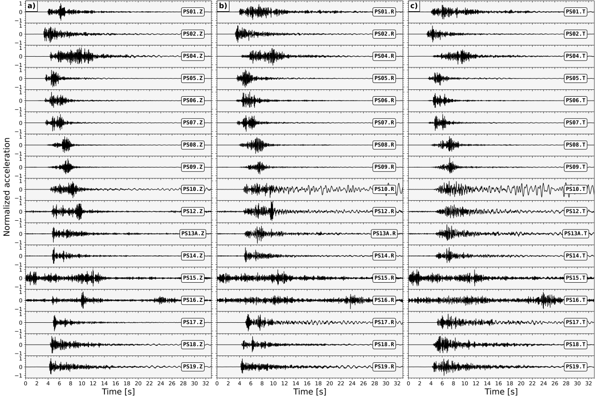
Figure 4: Seismograms induced by the explosion S4 (charge weight of 680 kg TNT-equivalent) and recorded by the seismic stations: (a) vertical component, (b) radial component, (c) transverse component. The traces are 20 Hz lowpass filtered. Note the significant variability in the signal duration (site PS10 with respect to site PS06, for instance). See Figure 1 for the station map.
