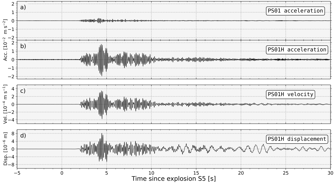
Figure 12: Comparison of the seismic signals (transverse component of the seismograms) at the station PS01 (floor of the church) and the station PS01H (bell tower) for the explosion S5 (charge weight of 600 kg TNT-equivalent). (a) Acceleration of the ground at PS01. (b) Acceleration of the ground at PS01H. Note the amplification of the motion between the floor and the bell tower. (c) Velocity of the ground at the station PS01H and (d) Displacement of the ground at the station PS01H.
