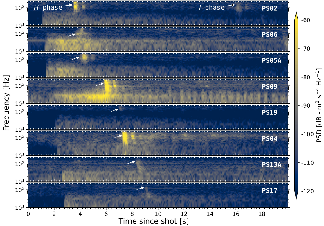
Figure 7: Spectrograms obtained from the vertical component of the signals generated by the explosion S8 (charge of 80 kg TNT-equivalent weight located at the site 3TY in the water column) and recorded by the MEMS accelerometers. The spectrograms are ordered as a function of the epicentral distances. The white solid arrows indicate the onset of the H -phase and the white open arrow indicates the onset of the acoustic phase ( I -phase). The spectrograms are computed over time windows of 0.2 s with 90% overlap.
