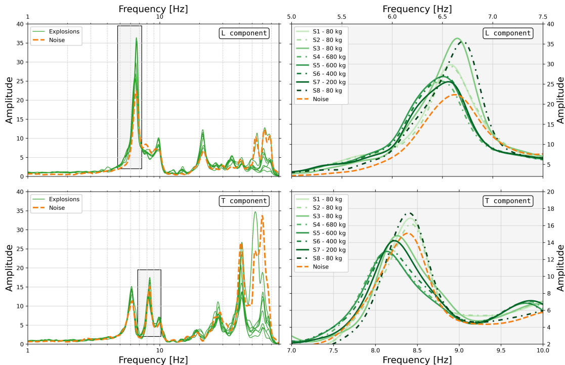
Figure 13: Transfer functions of the Sainte-Anne church to the solicitations of seismic waves generated by the UXO detonation (green curves) and by the environmental seismic noise (orange curves). (top row) Transfer functions along the longitudinal direction (along the nave of the church) and (bottom row) along the transverse direction. (left column) Transfer functions between 1 and 50 Hz. The grayed rectangles correspond to the extent of the panels on the right. (right column) Zoom on the single peak where the non-linear response of the building can be illustrated. The position of the peaks with respect to the full transfer function is indicated by the boxes on the left panels.
