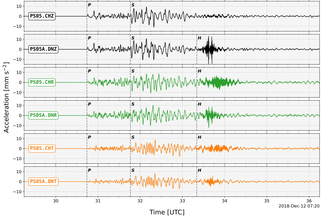
Figure 6: Comparison of acceleration traces induced by the explosion S4 (detonated at the site 3TY) and recorded at the collocated sensors PS05 (velocimeter) and PS05A (MEMS accelerometer). The black traces are the vertical components, the green traces are the radial components and the orange traces are the transverse components. The origin time corresponds to the estimated origin time for the explosion S4, i.e. 2018-12-12T07:20:29.5 (see section Inversion of onset times to better infer source locations and explosion times ). The dashed vertical gray lines correspond to the approximate time arrivals of P -, S - and H -phases, respectively.
