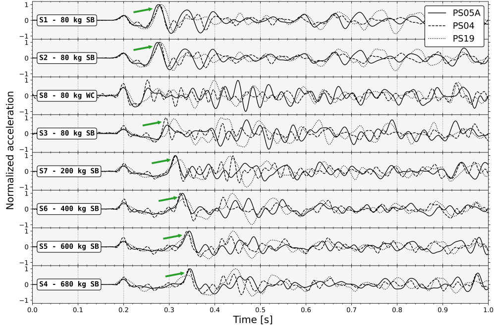
Figure 8: Detail of one second of the signal that includes the P -wave onset (at 0.2 s) generated by the explosions S1-S2 (located at the site 3TZ) and by the explosions S3-S8 (located at the site 3TY), and recorded at the stations PS05A (solid), PS04 (dashed) and PS19 (dotted). The vertical component of the seismograms is low-pass filtered at 50 Hz and the amplitudes are normalized. The green arrows highlight a phase whose delay seems correlated to the charge weights.
