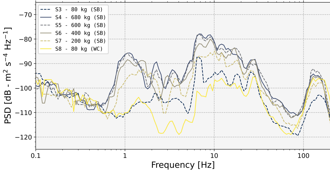
Figure 10: Power spectral densities of the seismic signals recorded at the station PS05A (vertical component) and induced by the explosions S3-S8 at the site 3TY. SB and WC refer to the configuration of the explosions, namely on the sea bottom and in the water column, respectively.
