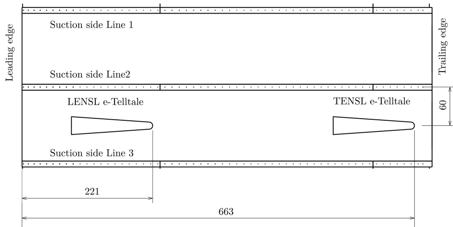
Figure 6. Positions of LENS and TENS e-TellTale sensors.
