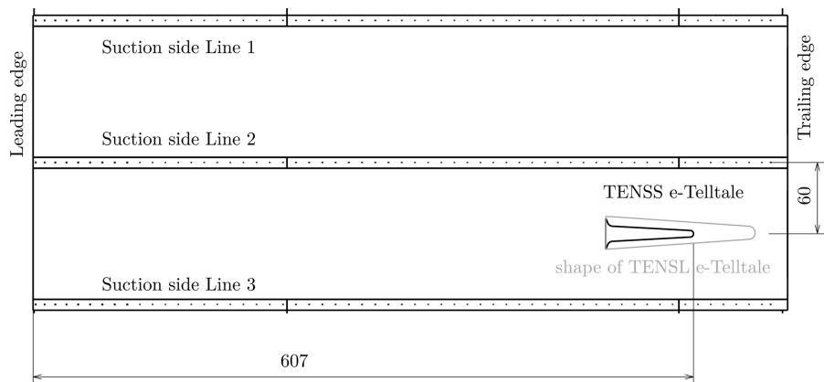
Figure 7. Position of the TENS e-TellTale.
