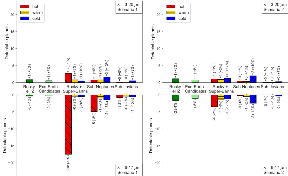
Fig. C.6. Impact of the wavelength coverage on the exoplanet detection yield. The numbers are relative to those shown for the reference scenarios with \lambda = 4\text{--}18.5\text{ }\mu\text{m} in Fig. 4. Left: scenario 1, with \lambda = 3\text{--}20\text{ }\mu\text{m} in the top panel and \lambda = 6\text{--}17\text{ }\mu\text{m} in the bottom panel. Right: scenario 2, with \lambda = 3\text{--}20\text{ }\mu\text{m} in the top panel and \lambda = 6\text{--}17\text{ }\mu\text{m} in the bottom panel.
