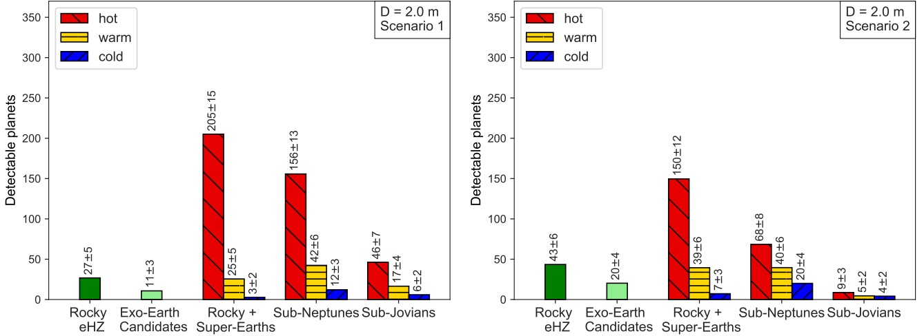
Fig. 4. Total exoplanet detection yield from our reference case scenario simulations ( D = 2 m; \lambda = 4\text{--}18.5\ \mu\text{m} ) using the planet classification scheme introduced by Kopparapu et al. (2018) (see Table 2). For comparison, we also plot the number of terrestrial exoplanets within the eHZ as defined in Sect. 2.6 as the leftmost bar labeled “Rocky eHZ.” The bars show the number of expected planet detections, including the statistical 1\text{-}\sigma uncertainty from the Monte Carlo approach but excluding uncertainties in the exoplanet occurrence rates. Left panel: scenario 1, i.e., the search phase is optimized for maximizing the total number of exoplanets. Right panel: scenario 2, i.e., the search phase is optimized for maximizing the number of rocky eHZ exoplanets.
