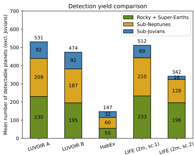
Fig. 11. Detection yield comparison between LUVOIR A/B , HabEx , and LIFE. For LIFE, we show the numbers for the D=2 m reference case and for HabEx the numbers from the baseline 4-m concept. Jovian planets are not shown, because they were not included in the LIFE simulations (cf. Sect. 2.2; see text for important details).
