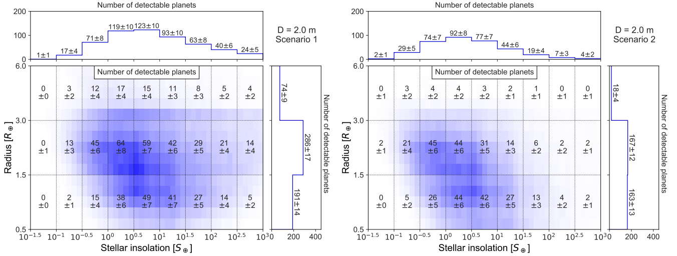
Fig. 3. Total exoplanet detection yield from our reference case scenario simulations ( D = 2 m; \lambda = 4\text{--}18.5\ \mu\text{m} ) in the radius vs. stellar insolation plane. The plots show the number of expected planet detections per grid cell, including the statistical 1\text{-}\sigma uncertainty from the Monte Carlo approach but excluding uncertainties in the exoplanet occurrence rates. Left panel: scenario 1 (search phase optimized for maximizing the total number of exoplanets). Right panel: scenario 2 (search phase optimized for maximizing the number of rocky eHZ exoplanets.)
