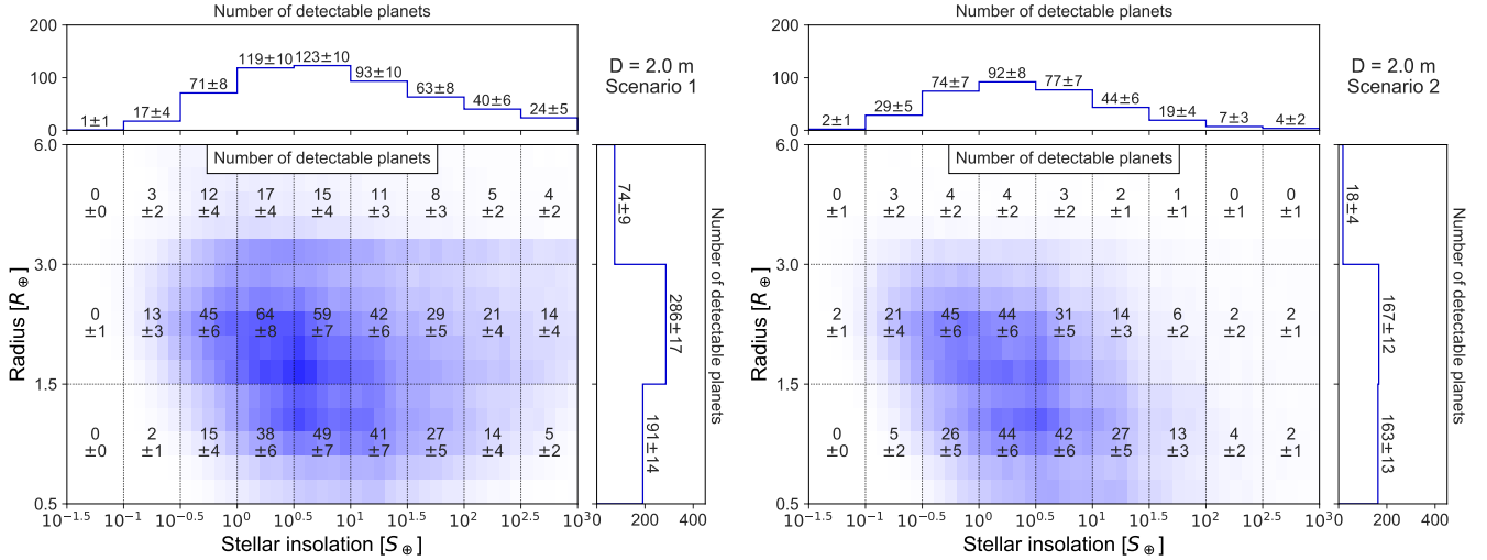
Fig. 3. Total exoplanet detection yield from our reference case scenario simulations ( D = 2 m; \lambda = 4\text{--}18.5 \mu\text{m} ) in the radius vs. stellar insolation plane. The plots show the number of expected planet detections per grid cell, including the statistical 1\text{-}\sigma uncertainty from the Monte Carlo approach but excluding uncertainties in the exoplanet occurrence rates. Left panel: scenario 1 (search phase optimized for maximizing the total number of exoplanets). Right panel: scenario 2 (search phase optimized for maximizing the number of rocky eHZ exoplanets.)
