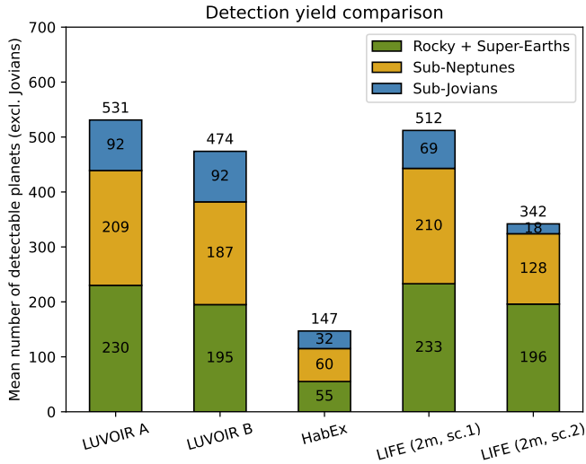
Fig. 11. Detection yield comparison between LUVUOIR A/B , HabEx , and LIFE . For LIFE , we show the numbers for the D = 2 m reference case and for HabEx the numbers from the baseline 4-m concept. Jovian planets are not shown, because they were not included in the LIFE simulations (cf. Sect. 2.2; see text for important details).
