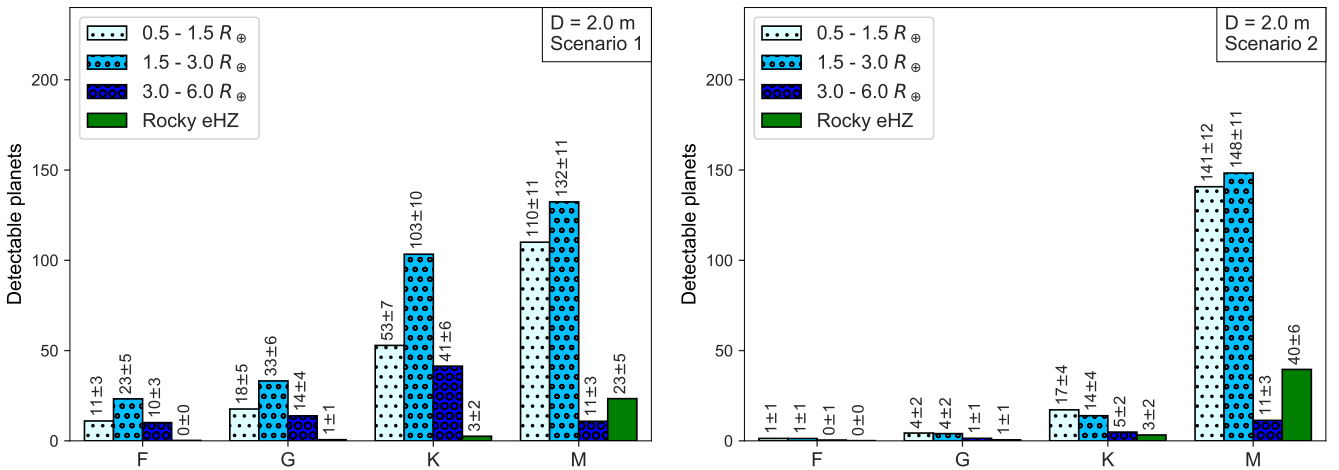
Fig. 5. Total exoplanet detection yield from our reference case scenario simulations ( D = 2 m; \lambda = 4\text{--}18.5\ \mu\text{m} ) shown as a function of spectral type of the host star ( left panel: scenario 1; right panel: scenario 2). The bars show the number of expected planet detections, including the statistical 1\text{-}\sigma uncertainty from the Monte Carlo approach but excluding uncertainties in the exoplanet occurrence rates. In both panels, the green bars (labeled “Rocky HZ”) show the number of rocky eHZ exoplanets, which are a subset of the planets in the 0.5\text{--}1.5\ R_{\oplus} bin in Fig. 3.
