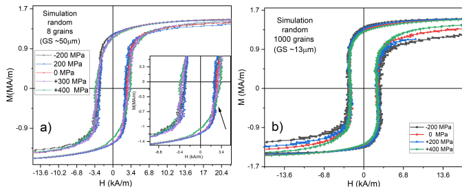
Figure 2: Hysteresis curves under uniaxial stress for random orientation of grains a) 8 grains; insert: zoom on the region where the curves cross; b) 1000 grains. The applied stress values are given in legend.
