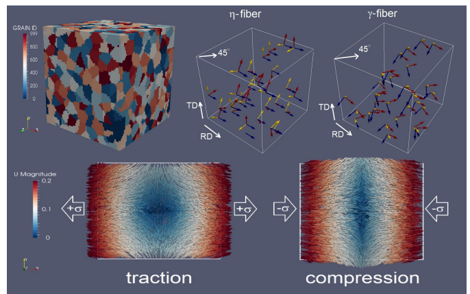
Figure 1: Top (from left to right): microstructure with 1000 grains, each grain has a different colour; crystallographic basic axis rotated in respect to RVE coordinate system for \eta -fiber and \gamma -fiber. Bottom: the displacement field distribution in case of tensile stress and compression.
