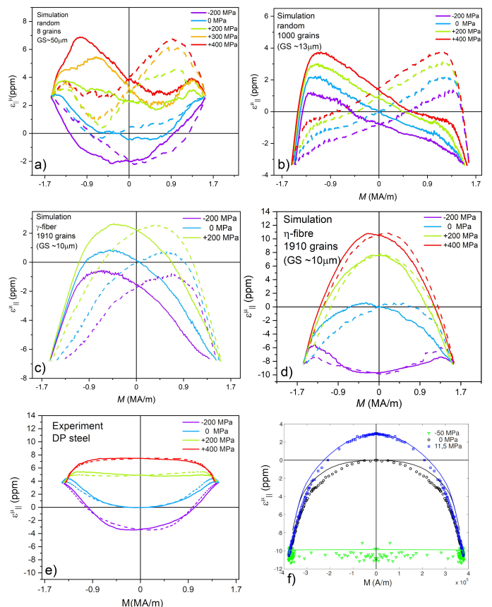
Figure 4: (a)-(d) Simulated longitudinal magnetostriction strain as a function of magnetization for a) randomly oriented 8 grains ; b) randomly oriented 1000 grains ; c) \gamma -fiber 1910 grains ; d) \eta -fiber 1910 grains. Solid lines correspond to the field sweep up, and dashed line - the field sweep down. (e)-(f) Experimentally measured longitudinal magnetostriction strain as a function of magnetization for e) DP steel ; f) ferrite NiZn (ahysteretic) [4]. Stress values are given in legends.
