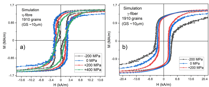
Figure 3: Hysteresis curves under uniaxial stress for a microstructure with 1910 grains (grain size \sim 10\mu\text{m} ) and a) \eta -fiber; b) \gamma -fiber. The applied stress values are given in legend.
