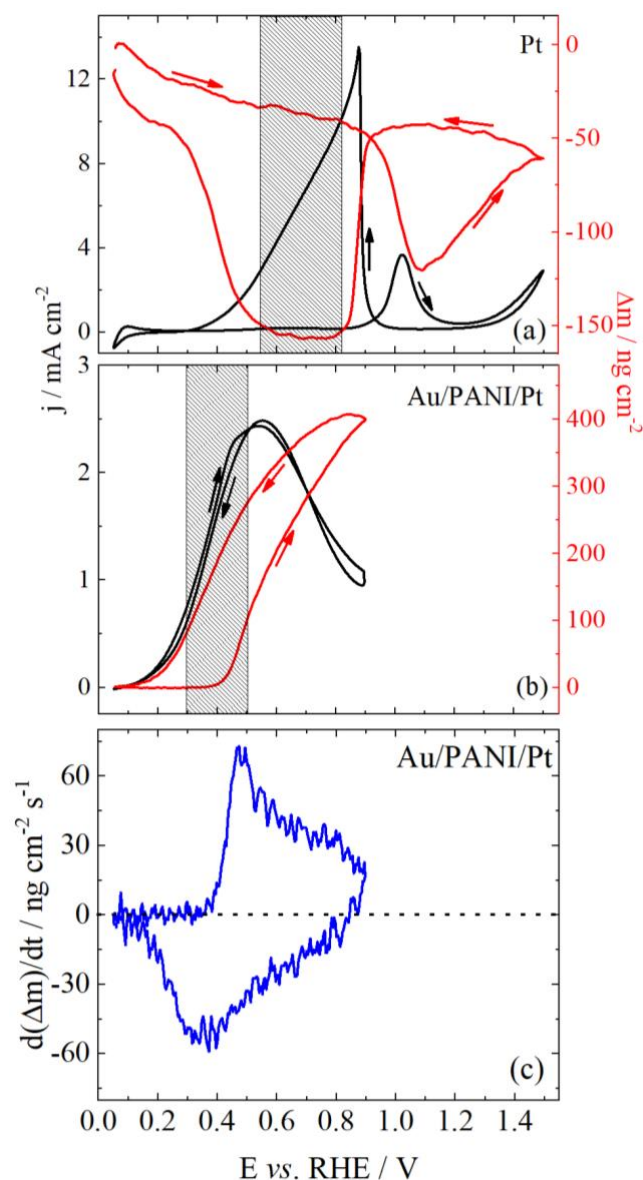
Figure 3: Voltammetric j/E and \Delta m/E profiles (recorded at 50 \text{ mV s}^{-1} ) for (a) Pt and (b) Au/PANI/Pt electrodes. (c) d(\Delta m)/dt vs. E for the mass variation profile given in (b). Electrolyte: aqueous solution containing 0.5 \text{ mol L}^{-1} \text{ H}_2\text{SO}_4 and 1 \text{ mol L}^{-1} \text{ HCOOH} . The current and mass were normalized (a) by the electroactive area (Pt hydrogen area, see text for details), and (b) by the geometric area, as in Figure 1.
