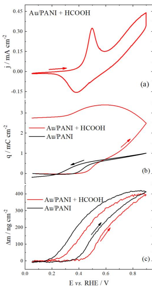
Figure 6: Voltammetric (a) j/E , (b) q/E , and (c) \Delta m/E profiles (recorded at 50 \text{ mV s}^{-1} ) for the Au/PANI modified electrode in the presence of 1 \text{ mol L}^{-1} HCOOH. q/E and \Delta m/E in the absence of HCOOH is also given for reference, see also Figure 1(a). Electrolyte: aqueous solution containing 0.5 \text{ mol L}^{-1} \text{H}_2\text{SO}_4 . Current and mass were normalized by the geometric area of the electrode.
