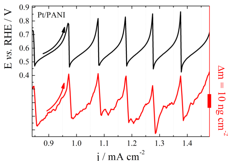
Figure 8: Galvanodynamic sweep ( 1.5 \mu\text{A s}^{-1} ) for the electro-oxidation of HCOOH on Pt/PANI electrode. Electrolyte: aqueous solution containing 0.5 \text{ mol L}^{-1} \text{ H}_2\text{SO}_4 and 1 \text{ mol L}^{-1} \text{ HCOOH} .
