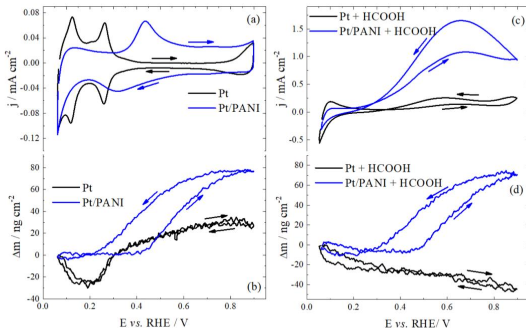
Figure 7: Voltammetric j/E and \Delta m/E profiles (recorded at 50 \text{ mV s}^{-1} ) in (a) and (b) aqueous solution containing 0.5 \text{ mol L}^{-1} \text{H}_2\text{SO}_4 , and (c) and (d) after addition of HCOOH ( 1 \text{ mol L}^{-1} ), for Pt (black) and Pt/PANI (blue) electrodes. Current and mass were normalized by the real area, as determined by the hydrogen region for the bare platinum electrode.
