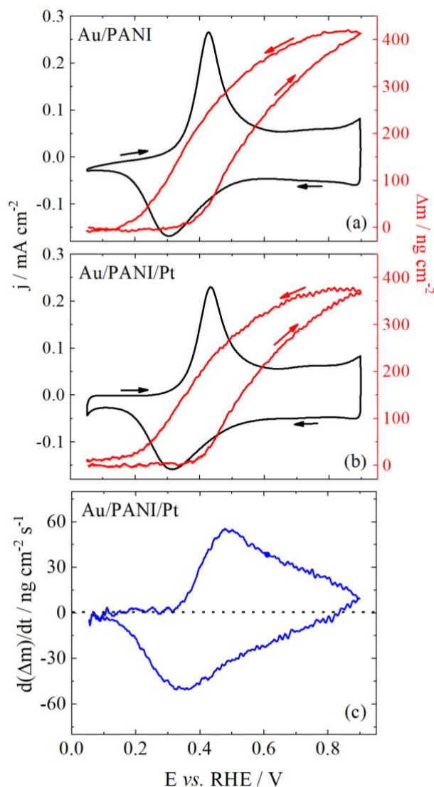
Figure 1: Voltammetric j/E and \Delta m/E profiles (recorded at 50 \text{ mV s}^{-1} ) for (a) Au/PANI and (b) Au/PANI/Pt modified electrodes. (c) d(\Delta m)/dt vs. E for the mass variation profile given in (b). Electrolyte: aqueous solution containing 0.5 \text{ mol L}^{-1} \text{H}_2\text{SO}_4 . Current and mass were normalized by the geometric area of the electrode.
