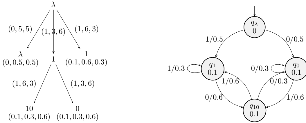
Figure 3: An n-ary classification tree (left), and the corresponding PDFA (right)
