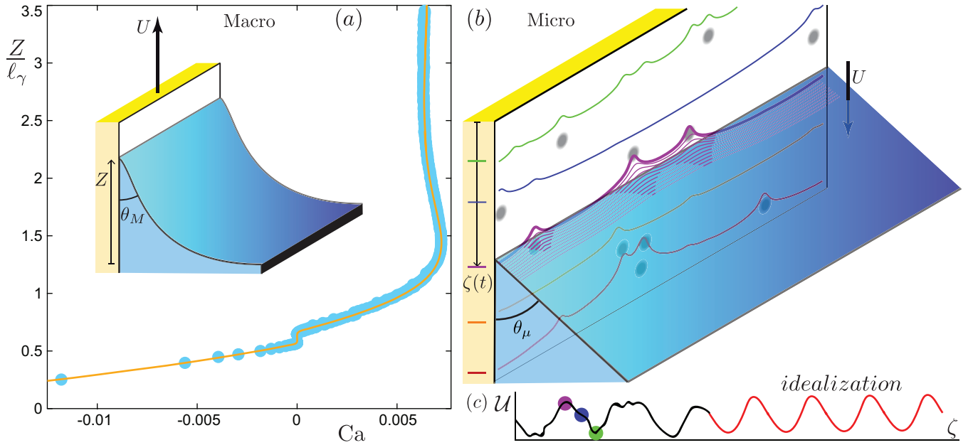
FIG. 1: (color online) (a) Height Z of the contact line as a function of the capillary number Ca , in the limit \dot{Z} \rightarrow 0 ( Z is rescaled by the capillary length l_\gamma = \sqrt{\gamma/\rho g} where \rho is the liquid density and g the acceleration of gravity). Circles: experimental data. Solid line: theory. Inset : schematic of the dip-coating experiment in the frame of reference of the bath. (b) Schematic of the contact line deformation over defects in the frame of reference of the plate. (c) Schematized energy landscape along the reaction path. Left: realistic Right: idealization.
