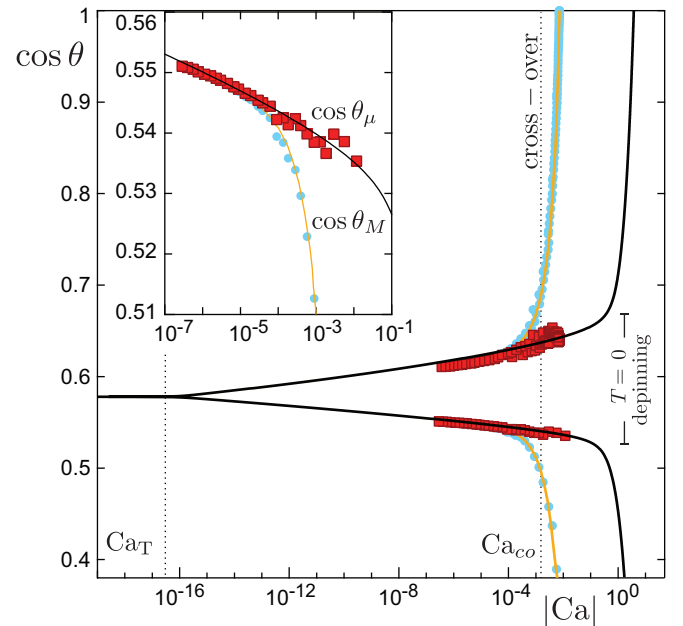
FIG. 2: Cosine of the free surface angle as a function of the capillary number \text{Ca} . Circles: experimental macroscopic angle \cos \theta_M = (Z/\ell_\gamma)\sqrt{1 - 0.25(Z/\ell_\gamma)^2} . Squares: experimental microscopic angle \cos \theta_\mu . Solid lines: theory for the microscopic angle and for the macroscopic angle. The depinning thresholds at zero temperature are indicated by arrows. Inset : close-up of the advancing branch ( \text{Ca} < 0 ).
