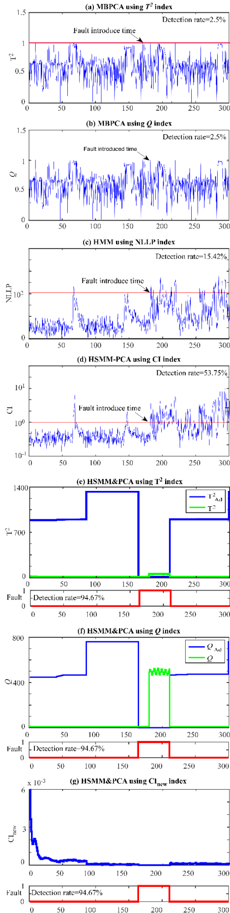
Fig. 7. Fault detection of Fault 9 data test
