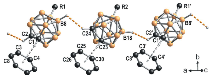
Figure 4 Intermolecular carborane–phenyl- \pi ( \text{CH} \cdots \pi\text{C}_6 ) interactions. [ R 1 = R 2 = \text{C}_6\text{H}_4\text{-N}(\text{CH}_2\text{-Ph})_2 ]. Symmetry codes as in Table 3 and x - 1, y, z .
