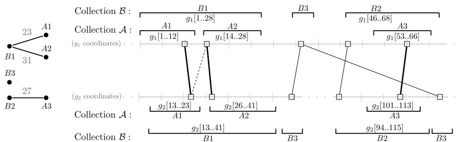
Fig. 1: To the right , the collections of blocks \mathcal{A} = \{A_1, A_2, A_3\} and \mathcal{B} = \{B_1, B_2, B_3\} appearing in genomes g_1 and g_2 , along with the graph BG(\mathcal{A}, \mathcal{B}) . Segments are depicted with brackets and lined up according to their positions on the chromosomes. They are labeled by their tuple (when space permits) and the block to which they belong. The configuration of positive and negative witness pairs shows that \mathcal{B} generalizes \mathcal{A} . Some of the genome positions are highlighted with boxes, and two such positions are connected by a solid line if they appear as a positive witness in \mathcal{B} , and that line is bold if they are also in \mathcal{A} . The dashed line represents one of the (many) negative homology witnesses between A_1 and A_2 that are negative witness pairs for \mathcal{A} but not for \mathcal{B} . To the left , the graph BG(\mathcal{A}, \mathcal{B}) appears with edges labeled by overlap length in gray. All of the connected components are stars.
