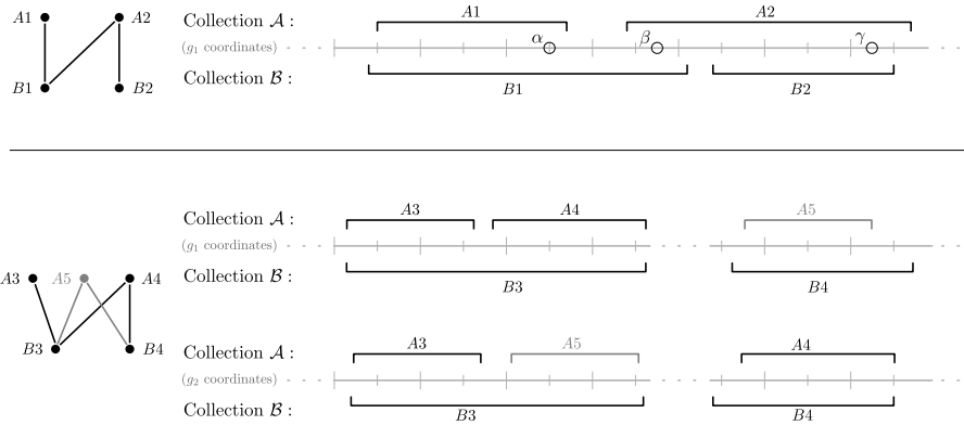
Fig. 2: Two subsets of blocks from collections \mathcal{A} and \mathcal{B} that are not hierarchically related. The top panel depicts a subset of blocks for part of the genome g_1 , but not the other genomes. Positions \alpha and \beta form a negative homology witness for \mathcal{A} , but not for \mathcal{B} , while \beta and \gamma form a negative homology witness for \mathcal{B} , but not for \mathcal{A} . This contradicts properties of a hierarchy and, therefore, yields the non-star topology to the left. The bottom panel depicts a subset of blocks for part of the genomes g_1 and g_2 . These segments contradict properties of a hierarchy in a different way, and yield the non-star topology to the left. This kind of scenario would arise when orthologs are matched in one way from MethodA, and in another way for MethodB. Note that even if the block A_5 was not in collection \mathcal{A} , the contradiction still holds and the connected component is not a star.
