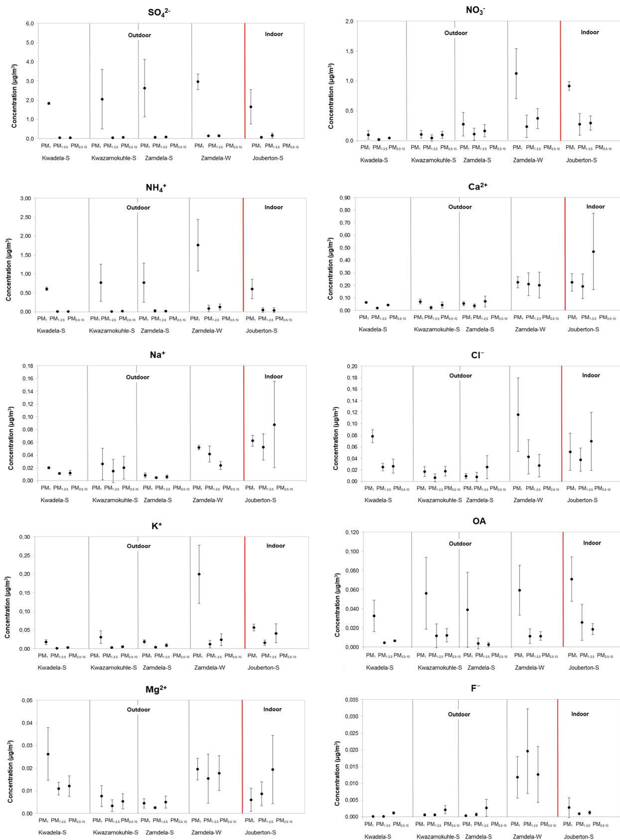
Figure 3. Mean concentrations ( \pm SD) of inorganic ionic species and water-soluble OAs measured in PM_1 , PM_{1-2.5} , and PM_{2.5-10} at each site during respective sampling campaigns.
