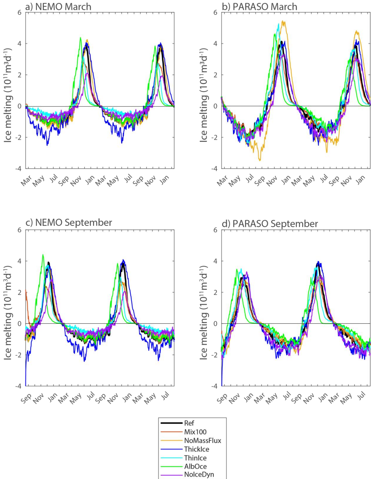
418 Figure 4. Mass flux due to sea ice growth and melt (counted positive for melting) integrated over 419 the Southern Ocean (in 10^{11} \text{ m}^3 \text{ d}^{-1} ) in the group of experiments starting in March (top row) and 420 September (bottom) for the NEMO (left column) and PARASO configurations (right column). This 421 diagnostic is evaluated online in NEMO from the different contributions to ice formation and melting 422 but is equivalent to the time derivative of the ice volume.
