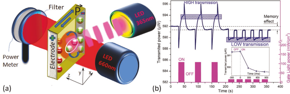
Figure 1. Optical control of light propagation. a) Schematic of the experimental setup with respect to the crystalline axis. b) Time dependence of the 660 nm beam transmission during periodic optical gating of 365 nm light. The inset shows a zoomed response of the depolarization regime limited by the LED response time (see text).
