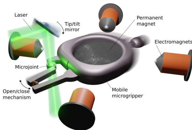
Fig. 1. Conceptual image of the proposed hybrid optothermal-magnetic mobile microgripper. The position of the microgripper is magnetically actuated and the gripping mechanism is optothermally actuated. The microgripper is approximately 1.5 mm in length.
