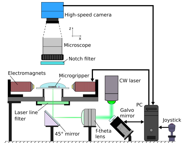
Fig. 3. Diagram of the experimental system and its components.
