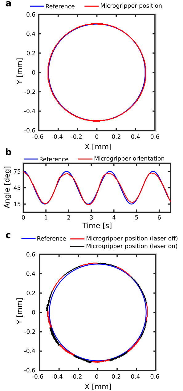
Fig. 6. Performance of the magnetic actuation system. (a) Path following of a circular trajectory. (b) Orientation control using a sinusoidal trajectory. The blue and red lines show the reference trajectory of the magnetic actuation and the position or orientation of the microgripper, respectively. (c) The effect of laser optothermal actuation on magnetic actuation showing the path following of the magnetically actuated microgripper while laser heating is applied periodically with a frequency of 0.5 Hz. The blue, red, and black lines show the reference trajectory of the magnetic actuation, the position of the microgripper in case of laser heating, the position of the microgripper in case of no laser heating, respectively.
