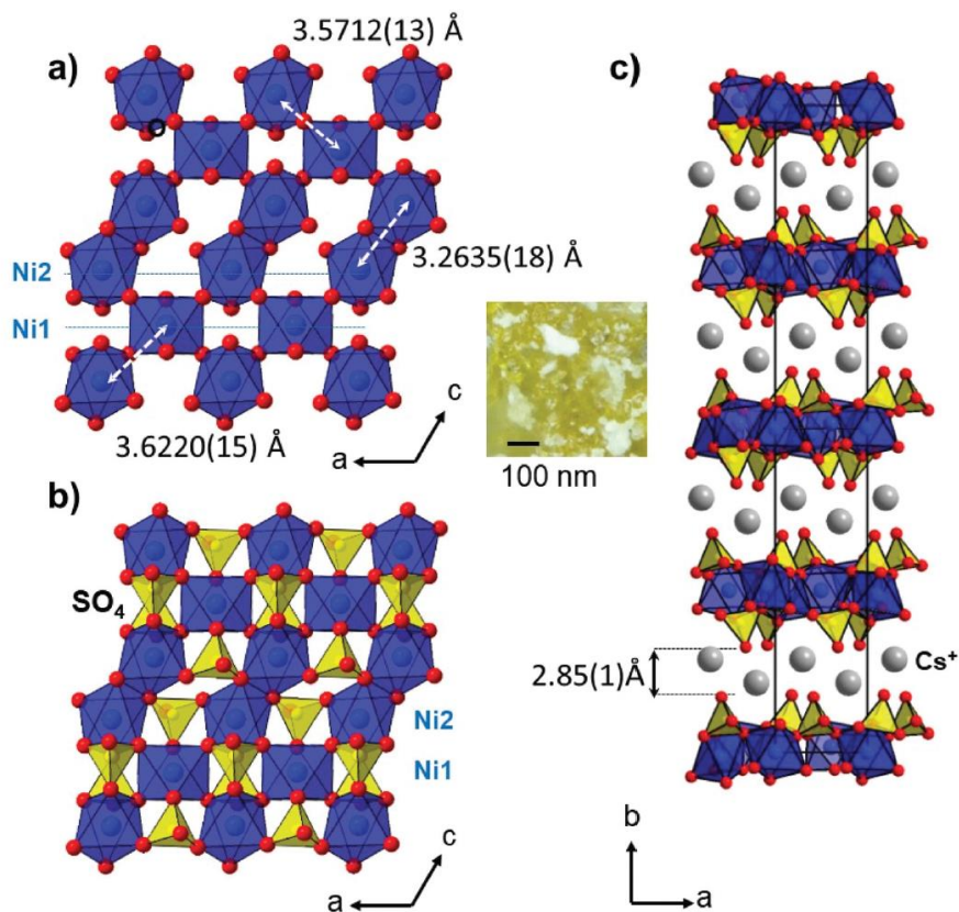
Fig. 1 2D blocks in 1 projected on the ac plane with (a) NiO 6 octahedra (blue) connected to (b) SO 4 tetrahedra (yellow) and (c) general projection of the crystal structure of 2 along the c -axis, showing the stacking and the interstitial Cs + cations (grey balls). The photo in the inset shows the color and shape of crystals.
