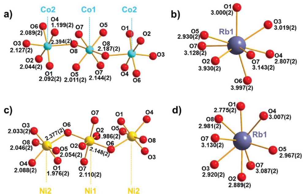
Fig. 5 \text{MO}_6 octahedra sharing corners giving \text{M}_3\text{O}_{16} trimers (a) in 4 ( M = \text{Co} ) and (c) in 3 ( M = \text{Ni} ) and \text{Rb}^+ environments (b) in 4 and (d) in 3. The cation–oxygen bond distances are given in Angströms.
