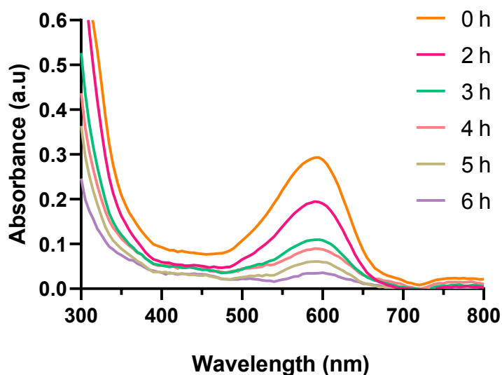
Figure 6. UV-Vis spectra of the NR-loaded NPs as incubated in 10 mM H 2 O 2 for 6 h at 37 °C.
