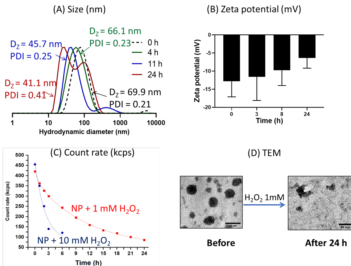
Figure 4. Characterization of spherical micelles of P- \text{M}_{45} in 1 mM \text{H}_2\text{O}_2 during 24 h. (A) Normalized intensity (%) as a function of size (nm) in DLS size distributions; (B) Zeta potential (mV) upon incubation with 1 mM \text{H}_2\text{O}_2 , (C) The exponential decrease of count rates of the same particle solution at 1 mg \text{mL}^{-1} when adding 10 mM or 1 mM \text{H}_2\text{O}_2 . Symbols are the experimental
