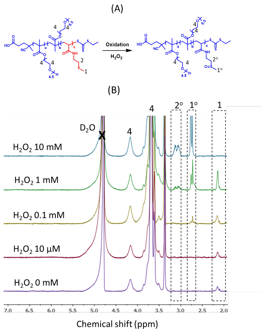
Figure 5. (A) Illustration of oxidative reaction of P-M 45 block copolymer NPs with H 2 O 2 ; (B) 1 H NMR spectra of P-M 45 at different concentrations of H 2 O 2 in D 2 O after 48 h.
