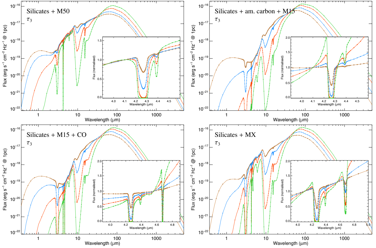
Fig. 8. Same as Fig. 7 but including the other models considered for the ice and core composition. Shown from the top left to the lower right are: silicate core, M50 ice mantle composition and size distribution \tau_3 , a_{\max} = 3\mu\text{m} (model #13); silicates and amorphous carbon core, M15 ice composition, and size distribution \tau_3 , a_{\max} = 3\mu\text{m} (model #16); silicate core, M15 ice mantle composition, including pure CO and size distribution \tau_3 , a_{\max} = 3\mu\text{m} (model #19); and silicate core, MX ice mantle composition, including H 2 O, CO 2 , CO, and NH 3 , and size distribution \tau_3 , a_{\max} = 3\mu\text{m} (model #22). The inserts display close-ups of the CO 2 ice band (and CO for models #19,22), with spectra normalised at 4.1 \mu\text{m} (4.55 \mu\text{m} for models #19,22).
