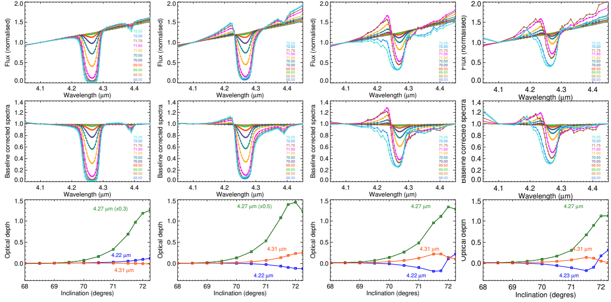
Fig. 14. Zoomed-in view of CO 2 spectra of the disk radiative transfer model with M15 ice mantle composition and MRN size distribution, a_{\max} = 0.25 \mu\text{m} (model #4); \tau_1 , a_{\max} = 1 \mu\text{m} (model #5); \tau_3 , a_{\max} = 3 \mu\text{m} (model #6); \tau_5 , a_{\max} = 5 \mu\text{m} (model #7); as observed at different disk inclinations. Top panels: flux spectra normalised at 4.1 \mu\text{m} . Middle panels: linear baseline corrected spectra with baseline reference points taken at 4.1 and 4.45 \mu\text{m} . Lower panels: evolution of the optical depth in the core (4.27 \mu\text{m} ), the blue wing (4.22 \mu\text{m} ), and red wing (4.31 \mu\text{m} ) with disk inclination.
