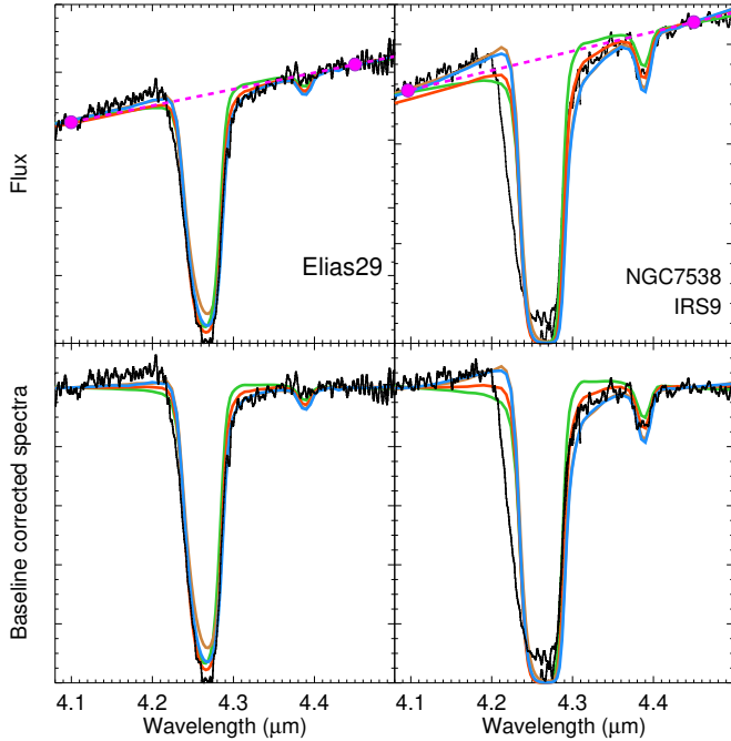
Fig. 13. Example of the comparison of two sources spectra with spherical clouds models. Upper panels: CO 2 anti-symmetric stretching mode observed fluxes with the ISO for Elias 29 and NGC7538 IRS9. A straight continuum baseline passing through points located at several times the band-FWHM from the band centre (magenta) is over-plotted, as well as spherical cloud radiative transfer models outputs for M15 mixture presented in Fig. 7 with different distribution upper size limits (MRN (green), \tau_1 (red), \tau_3 (blue), \tau_5 (brown)) scaled by an arbitrary (but common) factor for each observation. For Elias 29, the model spectra are for total visual extinction of 30. For NGC7538 IRS9, the model spectra are for total visual extinction of 60. Lower panels: same comparison but in transmittance, after baseline correction applied to each spectrum, which minimises baseline effects in the comparison.
