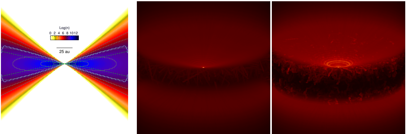
Fig. 9. Disk model and infrared images. Left panel: adopted disk model density distribution. The dashed lines show the hydrostatic scale height as a function of distance to the star responsible for the disk flaring. The cyan line defines the boundary of the region where ice mantles are present due to the visual extinction threshold. Middle and right panels: RADMC-3D radiative transfer code Monte Carlo images for MRN ( middle ) and \tau_3 ( right ) size distributions, ray traced at a wavelength of 4 \mu\text{m} , for the silicates + M15 ice mixture disk model, at an inclination of 72°.
