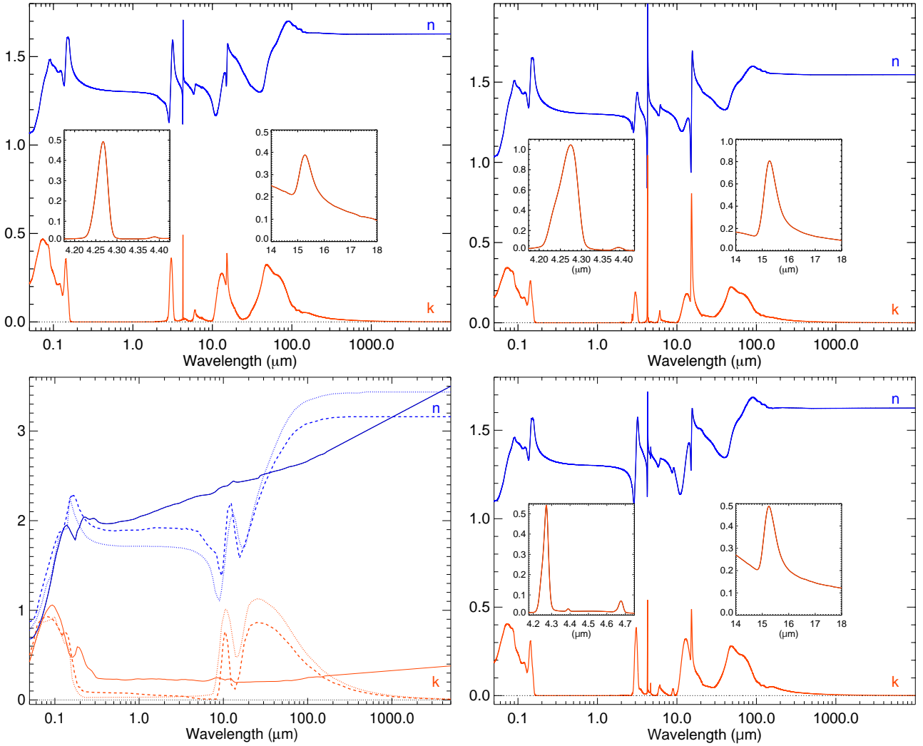
Fig. 1. Optical constants used in the models. Upper left: complex optical constants for the CO 2 :H 2 O 15:100 ice mixture (M15). Close-ups are shown for the imaginary part of the constant for the CO 2 stretching and bending modes. Upper right: complex optical constants for the CO 2 :H 2 O 50:100 ice mixture (M50). Close-ups are shown for the imaginary part of the constant for the CO 2 stretching and bending modes. Lower left: complex optical constants for the ‘astrosilicates’ (Draine & Lee 1984) and amorphous carbon AC1 from Rouleau & Martin (1991). Lower right: complex optical constants for the H 2 O:CO 2 :CO:NH 3 100:16:8:8 ice mixture. Close-ups are shown for the imaginary part of the constant for the CO 2 and CO stretching modes and CO 2 bending mode. See text for details.
