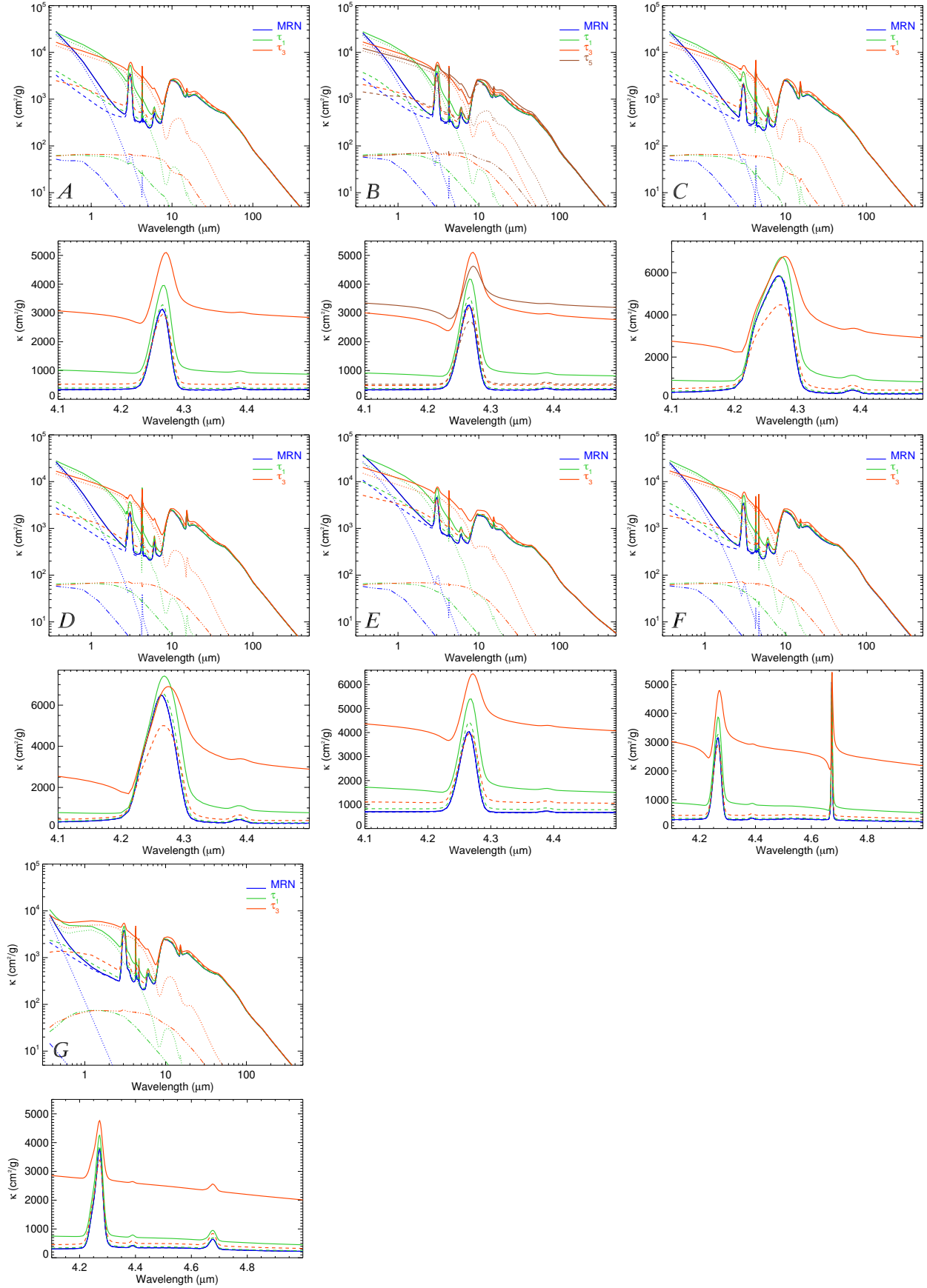
Fig. 6. Mass extinction coefficients (solid lines), absorption coefficients (dashed line), and Henyey–Greenstein phase function g (dot-dashed line, \times 100 ) for model sets A , B , C , D , E , F , and G (three models per panel corresponding to the MRN ( a_{\max} = 0.25\mu\text{m} ), \tau_1 ( a_{\max} = 1\mu\text{m} ), and \tau_3 ( a_{\max} = 3\mu\text{m} ) size distributions, respectively). Model set B includes a size distribution extending to \tau_5 ( a_{\max} = 5\mu\text{m} ). Below each panel a close-up of the CO 2 stretching mode is shown (which includes CO for the last two sets).
