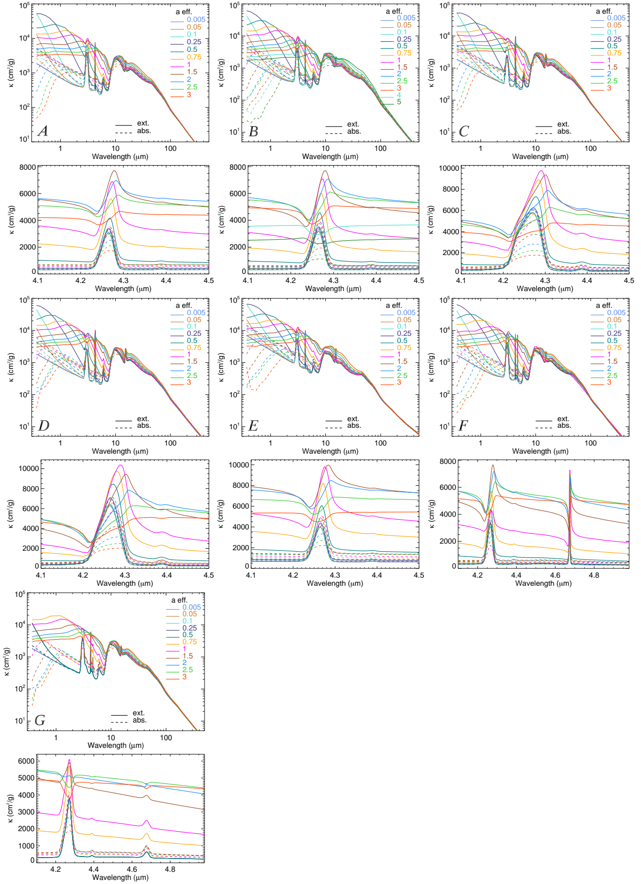
Fig. 5. Grain-size-dependent mass extinction coefficients (solid lines) and absorption coefficients (dashed line) for model compositions corresponding to model sets A, B, C, D, E, F, and G, from the upper left to the lower right, respectively. The mass extinction coefficients for increasing effective grain radius a_{\text{eff}} are shown. See text for details. For each set, a close-up of the CO 2 stretching mode is shown below it (for the last two panels, this also includes CO).
