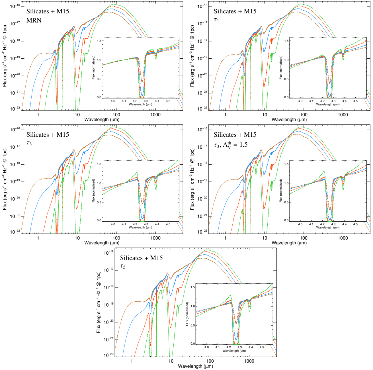
Fig. 7. Spectral energy distributions for the spherical radiative transfer for the M15 ice and core composition, with varying dust size distribution, for different visual extinctions ( A_V = 15 , brown; 30, blue; 60, red; 100, green). Distributions correspond to, from the top left to lower right: silicate core, M15 ice mantle composition and size distribution MRN, and a_{\max} = 0.25 \mu\text{m} (model #4); \tau_1 , a_{\max} = 1 \mu\text{m} (model #5); \tau_3 , a_{\max} = 3 \mu\text{m} (model #6); \tau_3 , a_{\max} = 3 \mu\text{m} (model #6) with ice threshold is set at A_V^{\text{th}}(\text{ice}) = 1.5 instead of 3; and \tau_5 , a_{\max} = 5 \mu\text{m} (model #7). The inserts display close-ups of the \text{CO}_2 ice band, with spectra normalised at 4.1 \mu\text{m} .
