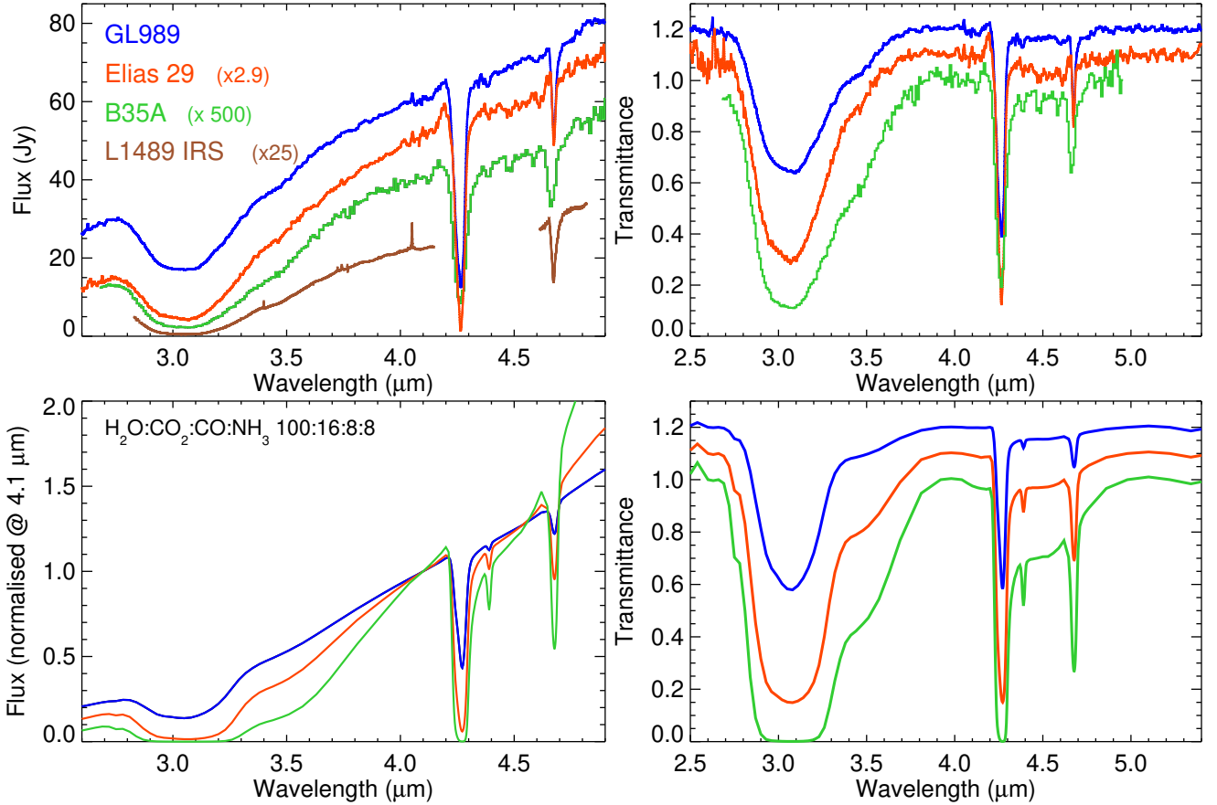
Fig. 16. Comparison between YSOs observations and models. Upper left: infrared observations in the H 2 O, CO 2 , CO stretching mode region for some sources with available coverage and for which gas-phase CO does not hamper observation of the CO ice profile. GL989 and Elias 29 are from the ISO database, B35A is an Akari spectrum (Noble et al. 2013), L1489 IRS is ground-based high resolution spectra from Boogert et al. (2002). In the L1489 spectrum, the gas-phase CO has been filtered out to show the CO ice profile. Lower left: spherical cloud model spectra with the MX mixture for a \tau_3 size distribution, for cloud visual extinction of A_v = 15 (blue), 30 (red), and 60 (green). The right panels show the same observations and models after baseline correction to provide transmittance spectra. The blue and red traces have been offset by 0.2 and 0.1, respectively, for clarity.
