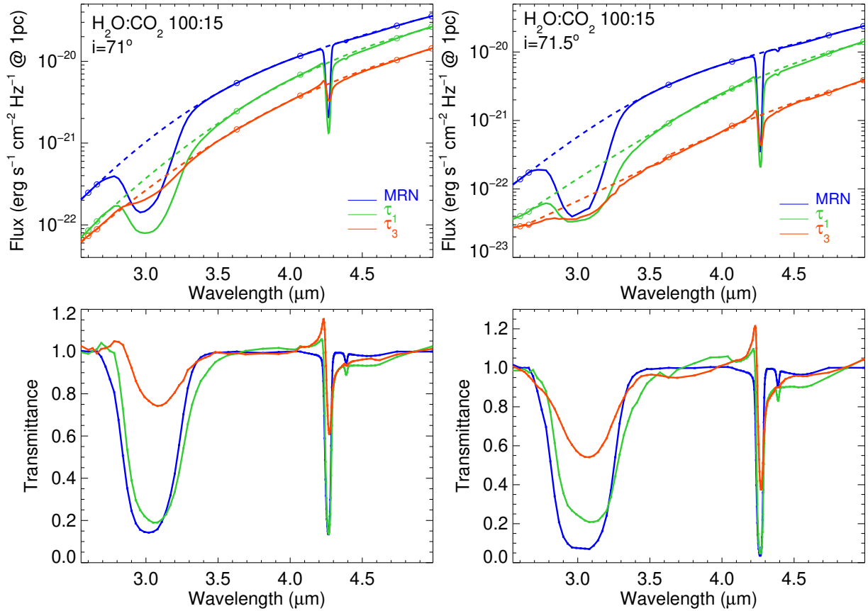
Fig. 15. Close-up of the disk radiative transfer models ( upper panels ) corresponding to silicates core, M15 ice mantle composition and size distribution MRN, a_{\max} = 0.25 \mu\text{m} (model #4); \tau_1 , a_{\max} = 1 \mu\text{m} (model #5); \tau_3 , a_{\max} = 3 \mu\text{m} (model #6); as observed under 71 and 71.5 degrees of inclination, in the water ice and carbon dioxide stretching modes range. A spline continuum passing through the indicated circle points, well apart from the core of the ice bands, is overlaid (dashed line). Lower panels show the extracted resulting transmittance spectra after dividing by this estimated continuum. In the highest optical depth spectrum ( i = 71.5^\circ , \tau_3 ) both the calculated spectrum and a slightly numerical noise filtered spectrum are shown. The asymmetry of the water ice band as well as the shift in the band centre are evidenced and accompanies the observed higher contrast CO 2 profile deformation.
