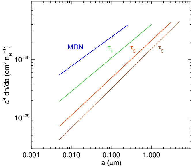
Fig. 4. Size distributions that qualitatively reproduce the expected size evolution behaviour for dust grain growth in aggregation models. The lower bound of the grain sizes is kept constant at 0.005 \mu\text{m} . The upper bound of the distribution is varied from 0.25 \mu\text{m} (MRN distribution) to 1 \mu\text{m} ( \tau_1 ), 3 \mu\text{m} ( \tau_3 ) and 5 \mu\text{m} ( \tau_5 ), and the slope is defined to maintain the same total mass. See text for details.
