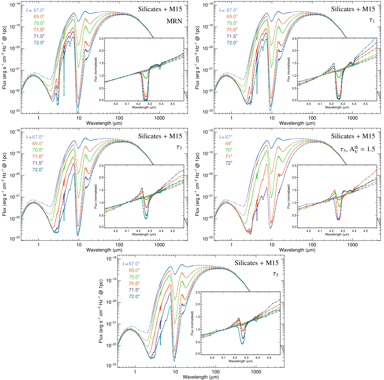
Fig. 10. Spectra of the disk radiative transfer model as observed under different disk inclinations for the M15 ice and core composition and different dust size distributions. Distributions correspond to, from the top left to the lower right : silicates core, M15 ice mantle composition and size distribution MRN, a_{\max} = 0.25 \mu\text{m} (model #4); \tau_1 , a_{\max} = 1 \mu\text{m} (model #5); \tau_3 , a_{\max} = 3 \mu\text{m} (model #6); \tau_3 , a_{\max} = 3 \mu\text{m} (model #6) with the ice threshold is set at A_V^{\text{th}}(\text{ice}) = 1.5 instead of 3; and a_{\max} = 5 \mu\text{m} (model #7).
