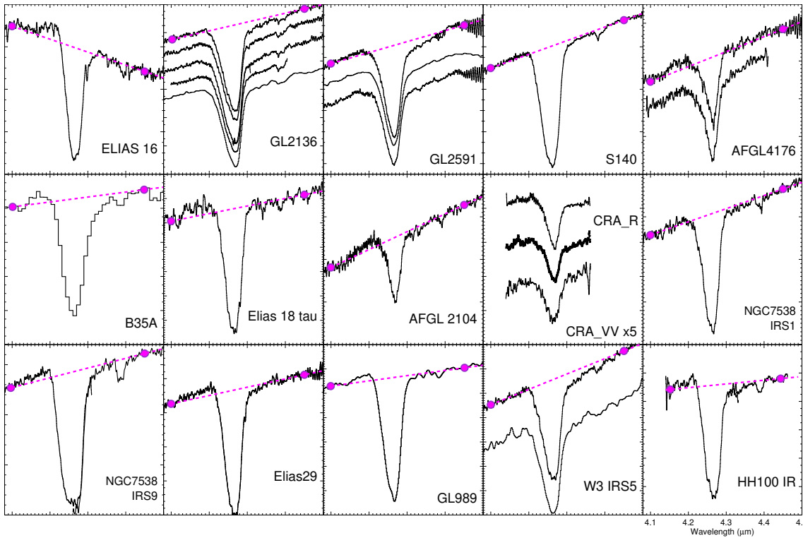
Fig. 12. Diversity of CO 2 anti-symmetric stretching mode observed fluxes with the Infrared Space Observatory (ISO) and Akari (source B35A) towards various astronomical lines of sight, including many massive protostellar objects. The profiles vary with some showing slightly warped asymmetric shapes (e.g. GL2591, B35A, Elias 29, GL989, HH100 IR, and NGC7538). A linear baseline passing through continuum points on each side, far from the band centre, indicated by circles, is plotted in each panel to show the various degrees of band asymmetry.
