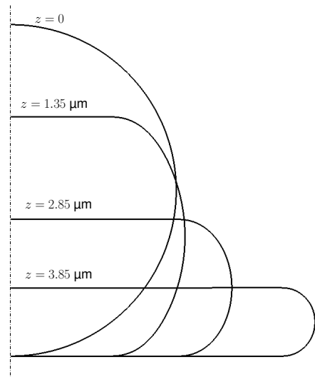
Figure 4: Initial and different deformed configurations of the spherical cell for the compressive loading at 2\ \mu\text{m/s} .
