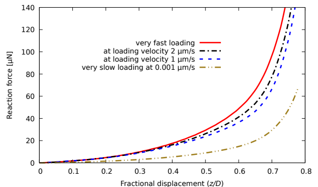
Figure 6: Compression of an ellipsoidal cell at different loading velocities.
