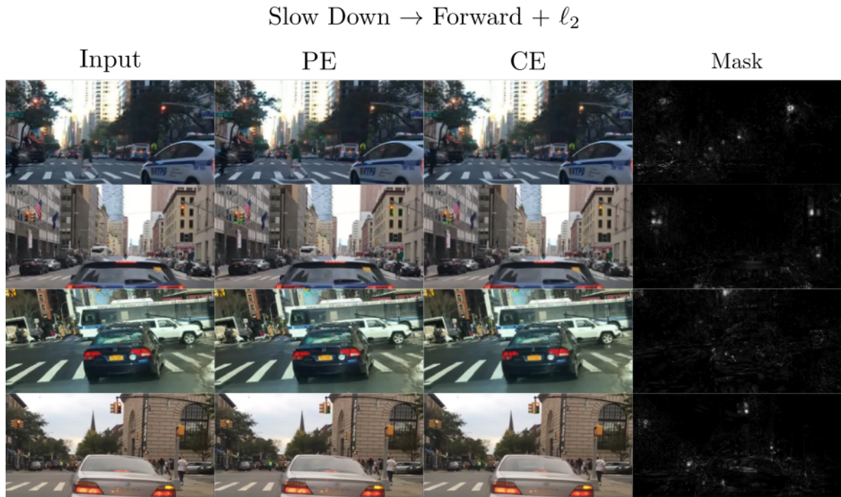
Figure 9. Additional BDD qualitative results. We show examples for the Forward / Slow Down binary class for \ell_2 distance loss. We show a zoom of the changes in the image since the perturbations are sparse. We see that ACE adds traffic light colors in the buildings to change the prediction.
