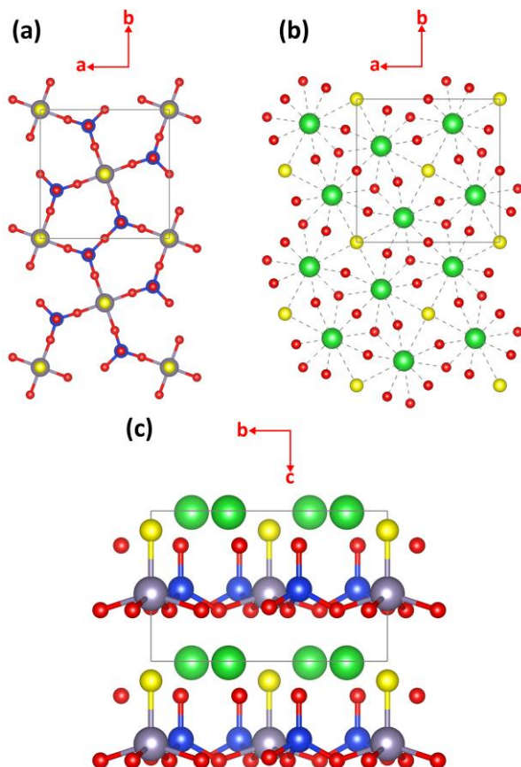
Figure 1. (a) A projection view of a SnSSi 2 O 7 layer along the c-axis. (b) A projection view of the coordination environment of the Ba 2+ ions. (c) A projection view of how the SnSSi 2 O 7 layers of Ba 2 SnSSi 2 O 7 are stacked along the c-direction with Ba 2+ ions lying in between them. The atoms are represented by colored spheres as follows: O = red, S = yellow, Si = blue, Sn = grey, and Ba = green.
