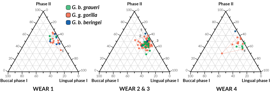
Figure 2. Ternary diagrams showing the proportions (in %) of relative wear areas of buccal phase I facets, lingual phase I facets, and phase II facets, which are positioned in an equilateral triangle. Each base of the triangle represents a ratio of 0% while the vertices correspond to a percentage of 100%. Tip crush areas were included in phase II facets. Gorilla beringei graueri in green, Gorilla gorilla gorilla in orange, and Gorilla beringei beringei in blue. Specimens 1 = AMNH 115609, 2 = AMNH 200506, 3 = SMF 59159, 4 = ZMB 47526, and 5 = BM 64.12.1.5.
