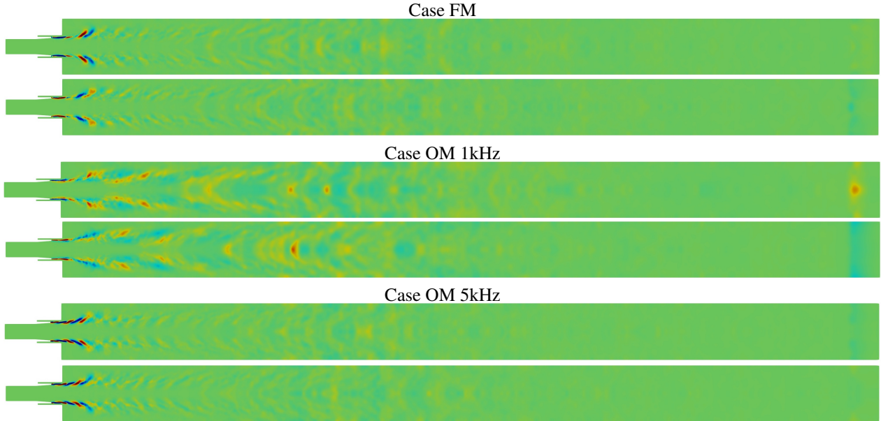
Figure 18: Longitudinal slices of phase-averaged heat release rate fluctuations (between -2 \cdot 10^{11} \text{ W/m}^3 and 2 \cdot 10^{11} \text{ W/m}^3 ) for \phi = 0 and \phi = \pi .
