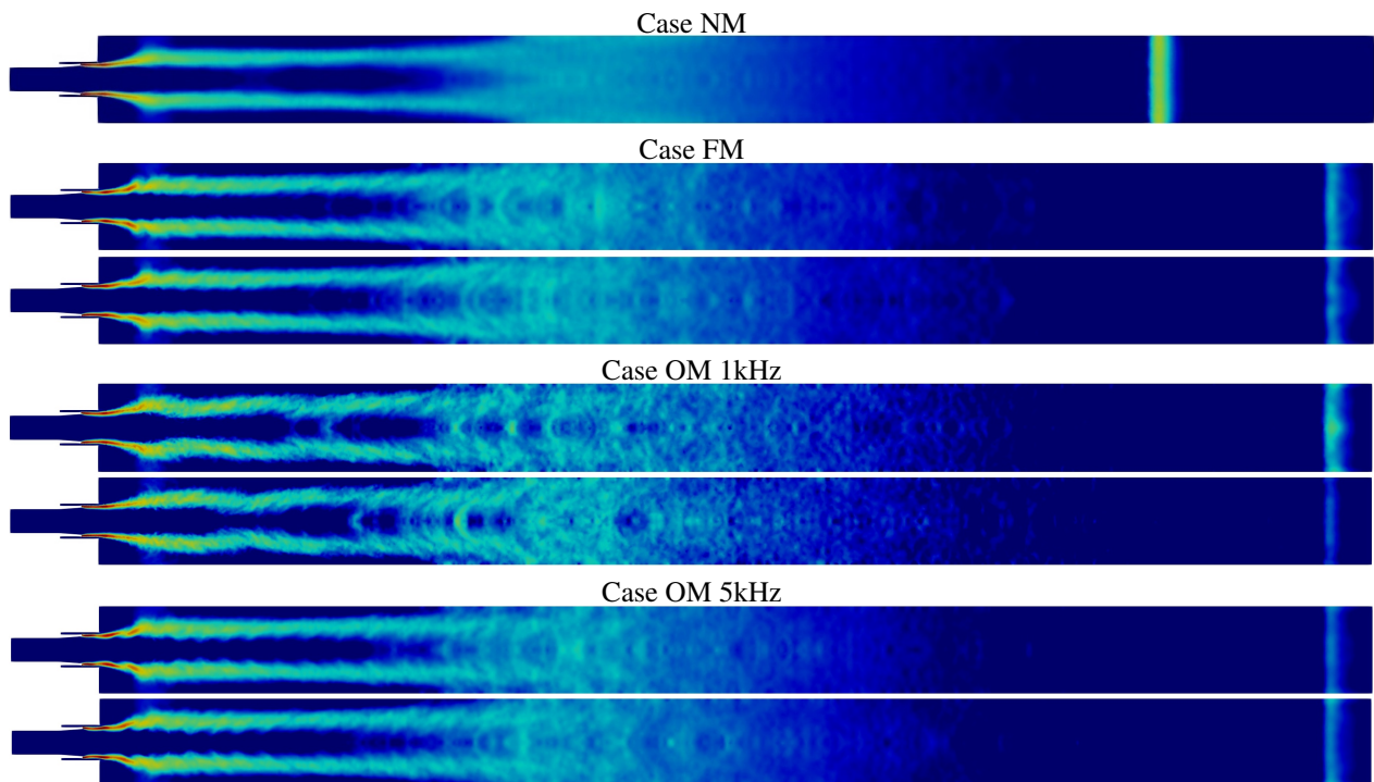
Figure 17: Longitudinal slices of phase-averaged heat release rate (between 2 \cdot 10^{10} W/m 3 and 2 \cdot 10^{12} W/m 3 ) for \phi = 0 and \phi = \pi .
